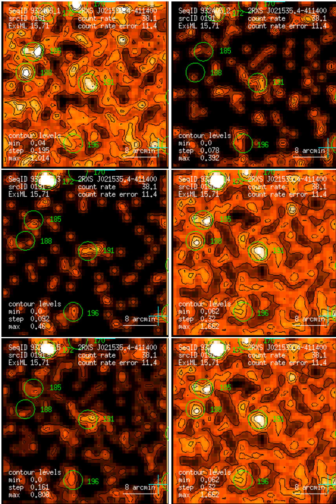
Figure 191: RASS 932405: detection 0191: band rate images, Gaussian filter: (1) PSPC channels 11 – 41, (2) 52 – 90, (3) 91 – 201, (4) 11 – 235, (5) 52 – 201, (6) 11 – 201. Broad band rates in counts/ks. Band rate contour levels in counts/ks/arcmin 2 .
