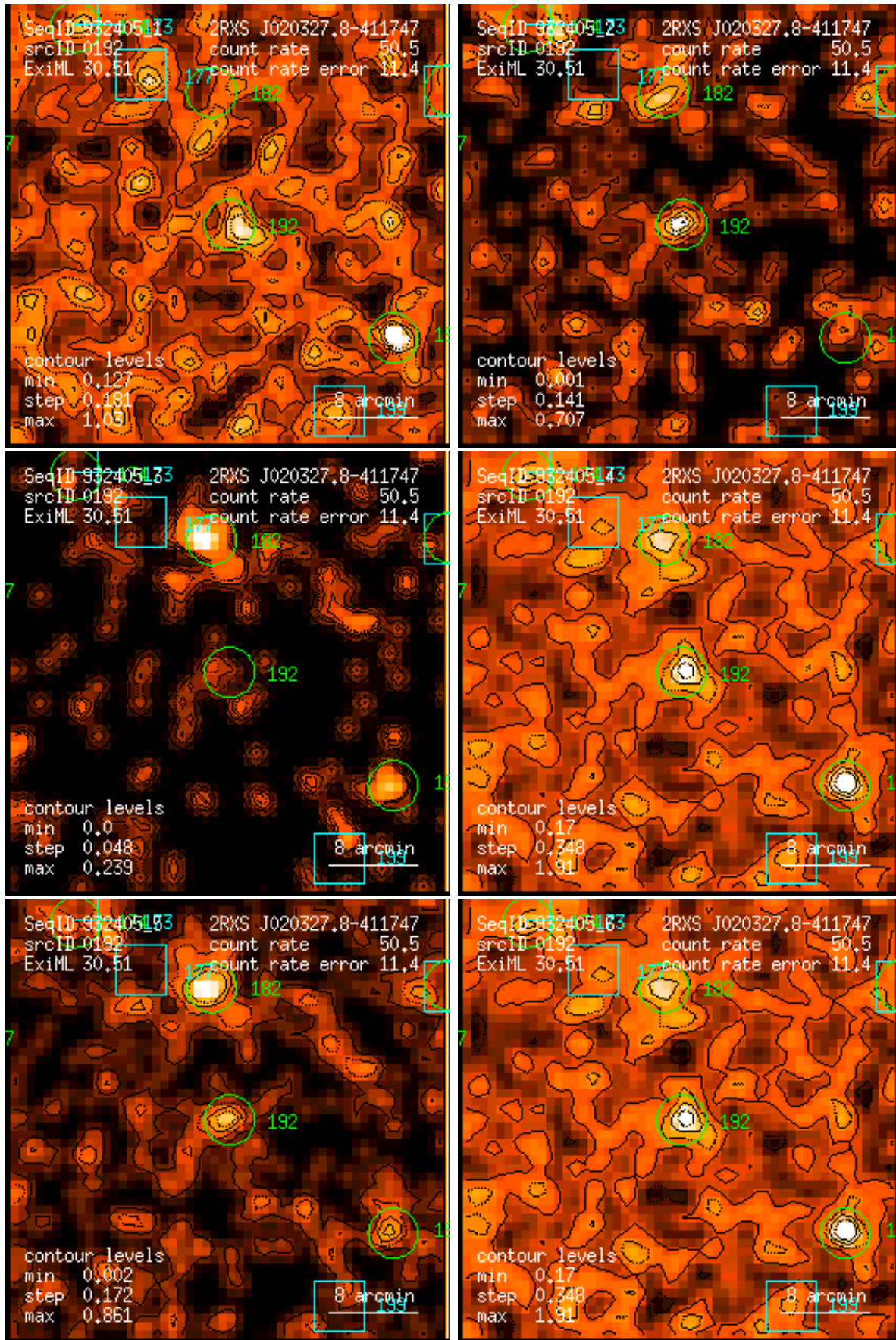
Figure 192: RASS 932405: detection 0192: band rate images, Gaussian filter: (1) PSPC channels 11 – 41, (2) 52 – 90, (3) 91 – 201, (4) 11 – 235, (5) 52 – 201, (6) 11 – 201. Broad band rates in counts/ks. Band rate contour levels in counts/ks/arcmin 2 .
