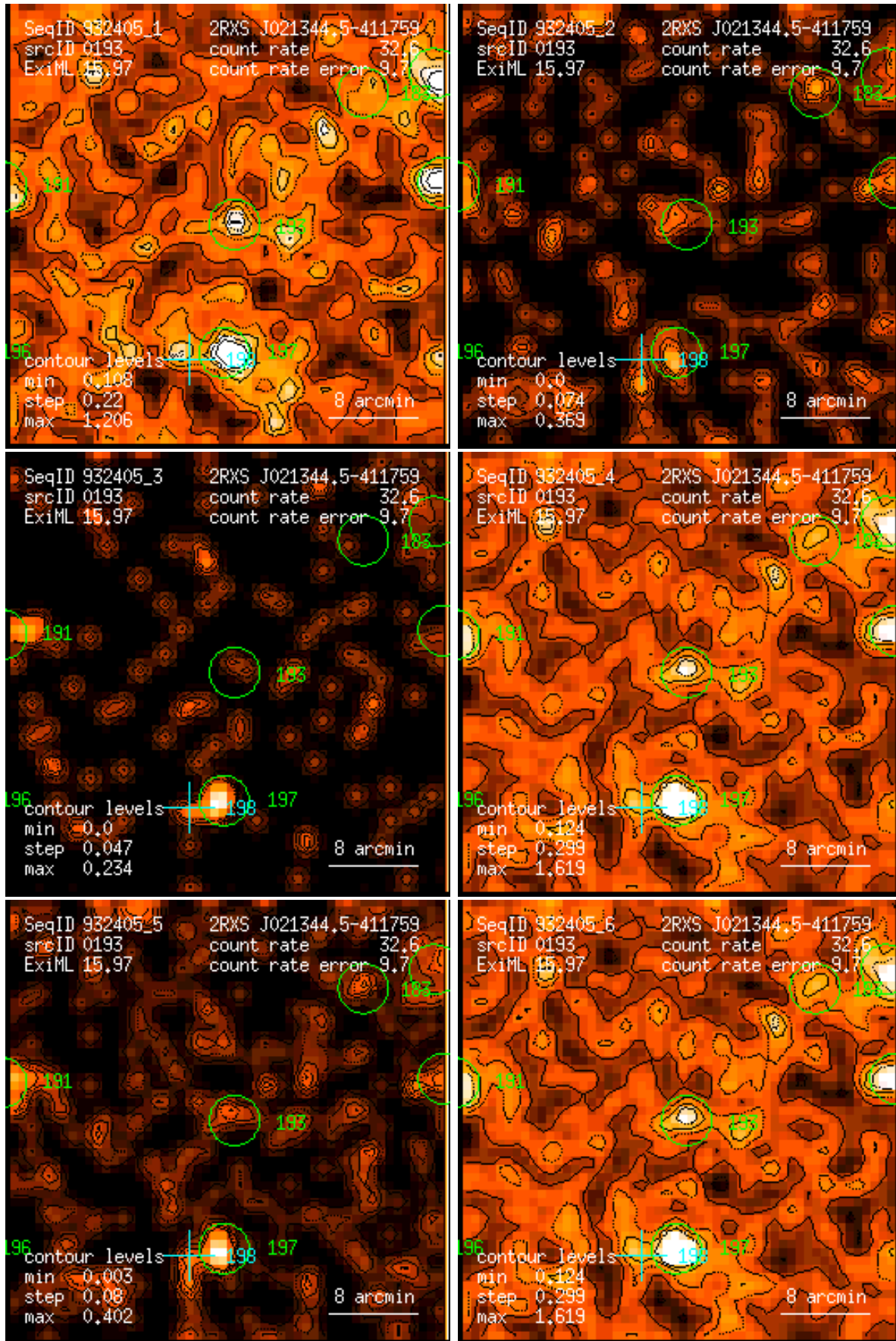
Figure 193: RASS 932405: detection 0193: band rate images, Gaussian filter: (1) PSPC channels 11 – 41, (2) 52 – 90, (3) 91 – 201, (4) 11 – 235, (5) 52 – 201, (6) 11 – 201. Broad band rates in counts/ks. Band rate contour levels in counts/ks/arcmin 2 .
