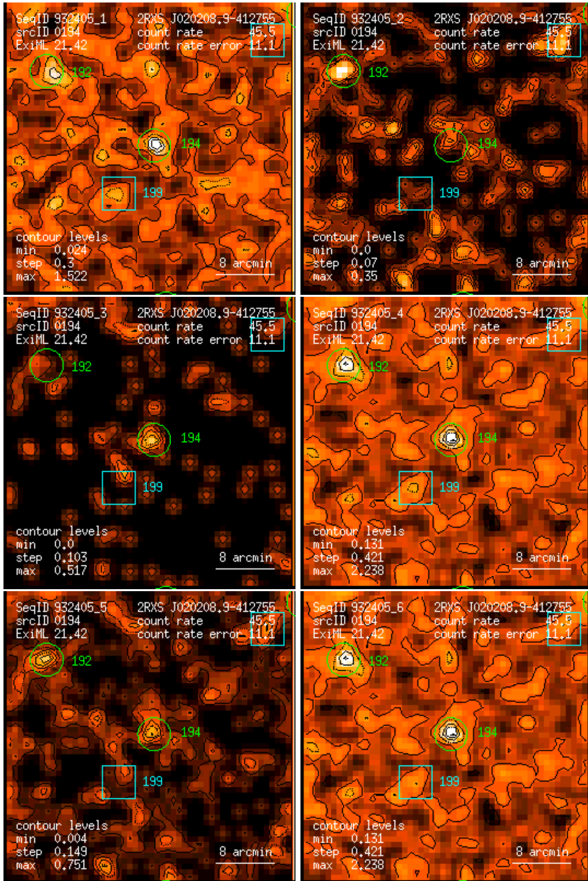
Figure 194: RASS 932405: detection 0194: band rate images, Gaussian filter: (1) PSPC channels 11 – 41, (2) 52 – 90, (3) 91 – 201, (4) 11 – 235, (5) 52 – 201, (6) 11 – 201. Broad band rates in counts/ks. Band rate contour levels in counts/ks/arcmin 2 .
