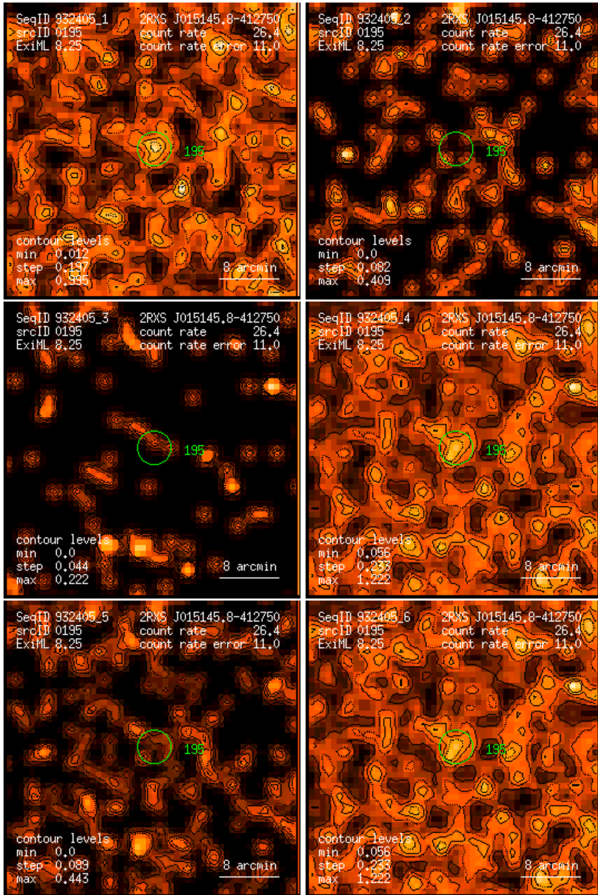
Figure 195: RASS 932405: detection 0195: band rate images, Gaussian filter: (1) PSPC channels 11 – 41, (2) 52 – 90, (3) 91 – 201, (4) 11 – 235, (5) 52 – 201, (6) 11 – 201. Broad band rates in counts/ks. Band rate contour levels in counts/ks/arcmin 2 .
