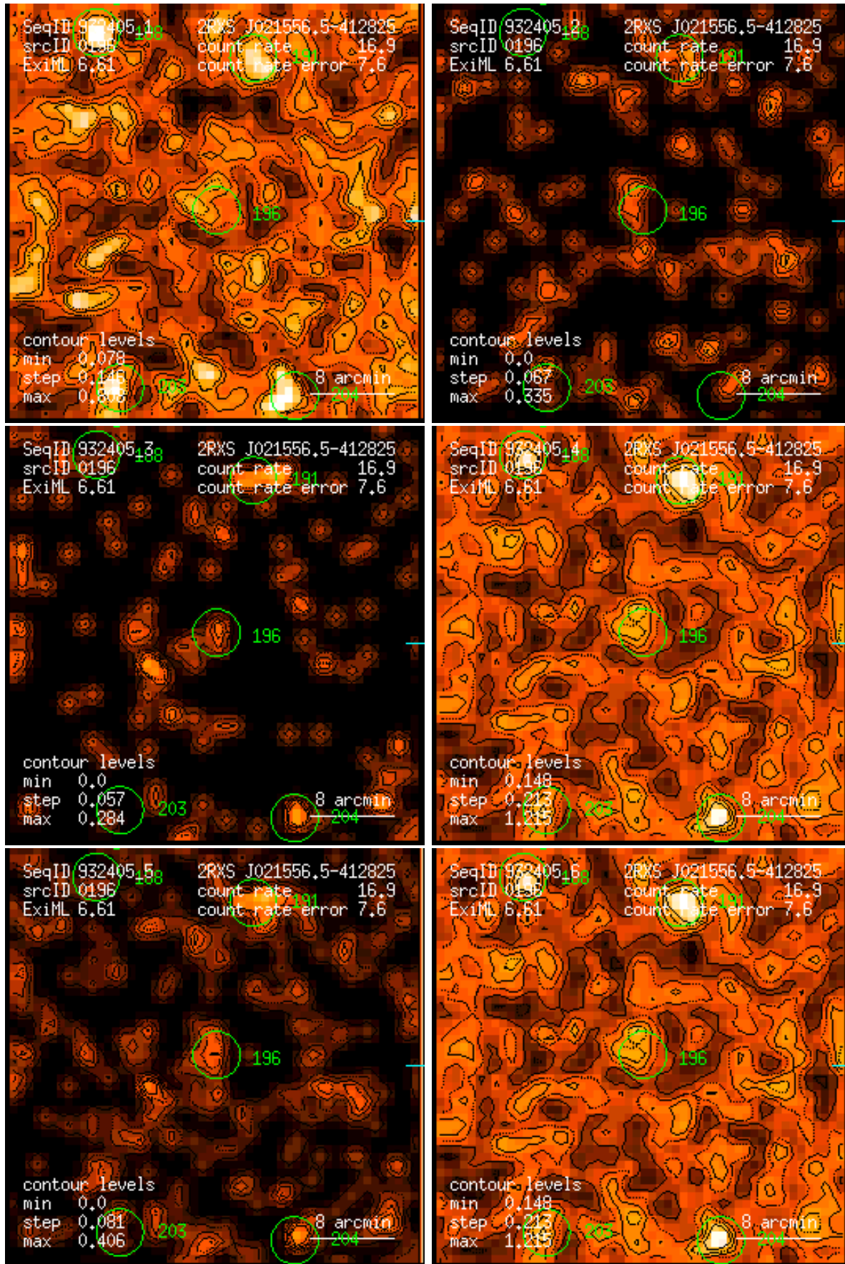
Figure 196: RASS 932405: detection 0196: band rate images, Gaussian filter: (1) PSPC channels 11 – 41, (2) 52 – 90, (3) 91 – 201, (4) 11 – 235, (5) 52 – 201, (6) 11 – 201. Broad band rates in counts/ks. Band rate contour levels in counts/ks/arcmin 2 .
