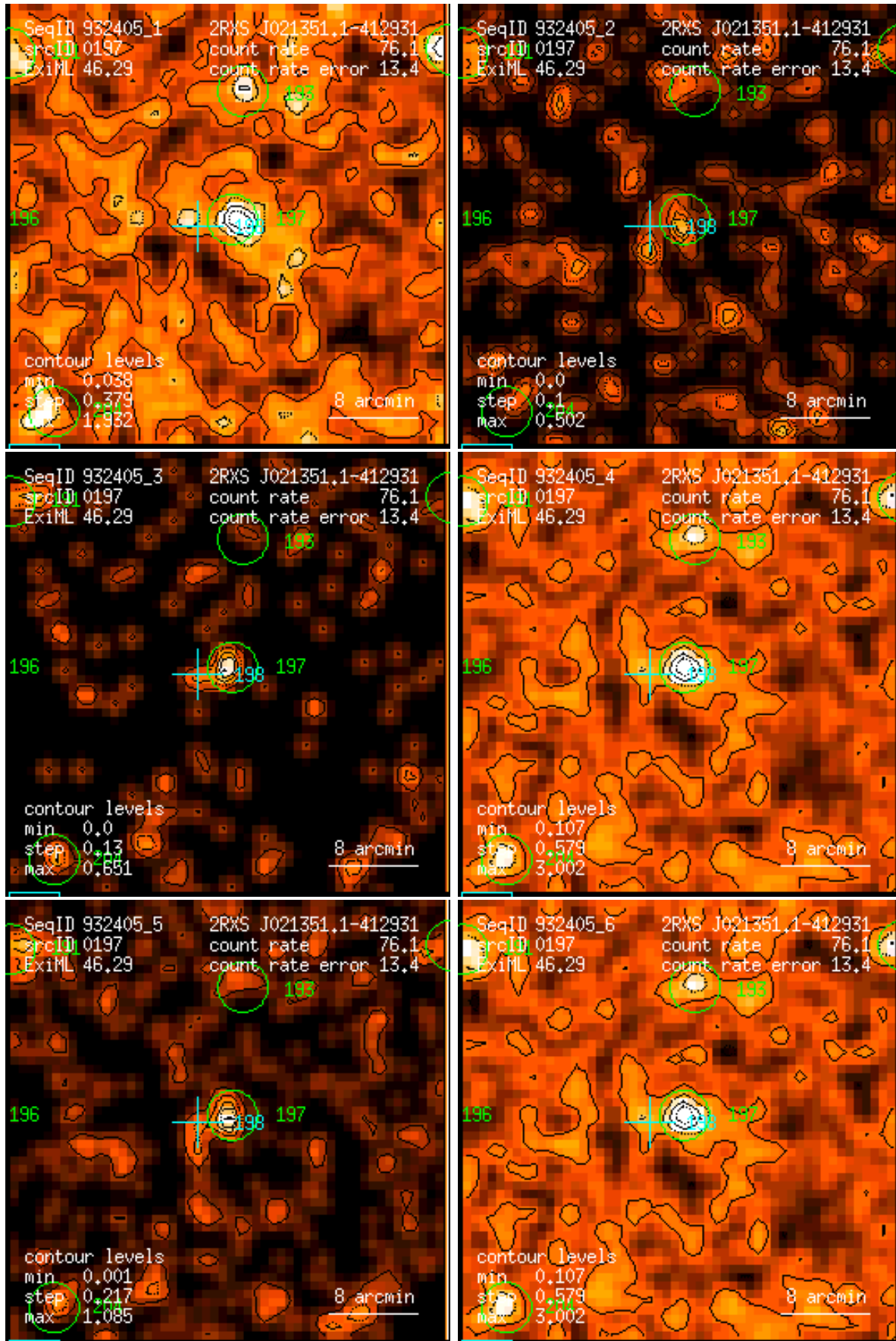
Figure 197: RASS 932405: detection 0197: band rate images, Gaussian filter: (1) PSPC channels 11 – 41, (2) 52 – 90, (3) 91 – 201, (4) 11 – 235, (5) 52 – 201, (6) 11 – 201. Broad band rates in counts/ks. Band rate contour levels in counts/ks/arcmin 2 .
