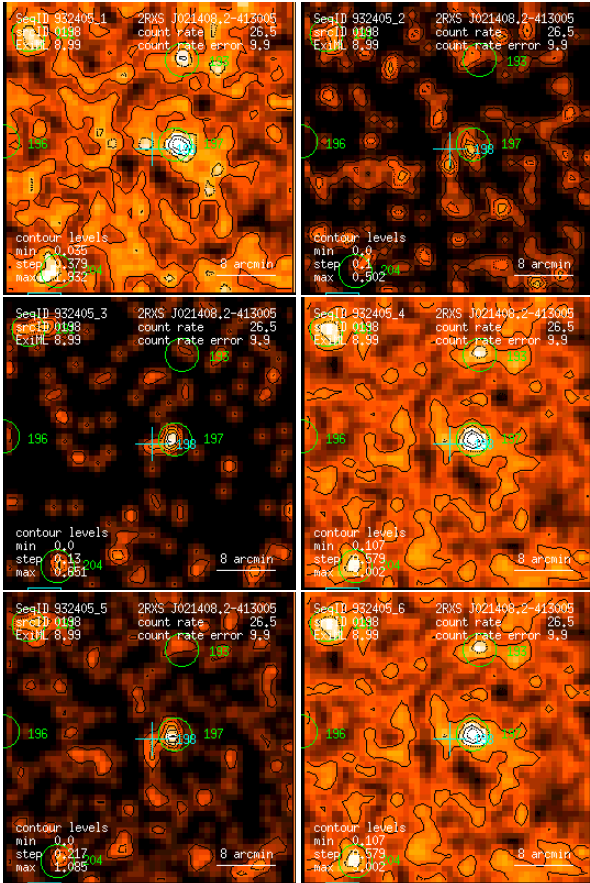
Figure 198: RASS 932405: detection 0198: band rate images, Gaussian filter: (1) PSPC channels 11 – 41, (2) 52 – 90, (3) 91 – 201, (4) 11 – 235, (5) 52 – 201, (6) 11 – 201. Broad band rates in counts/ks. Band rate contour levels in counts/ks/arcmin 2 .
