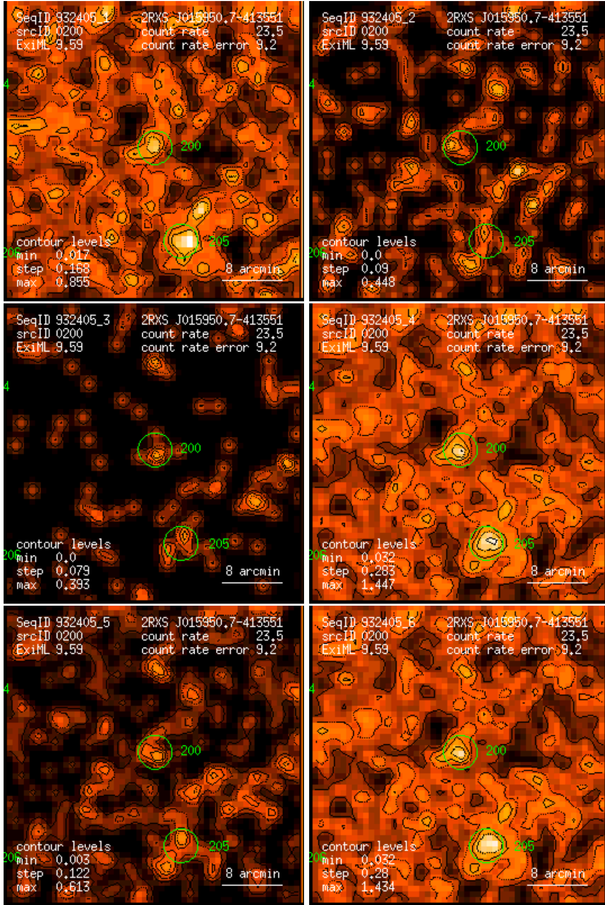
Figure 200: RASS 932405: detection 0200: band rate images, Gaussian filter: (1) PSPC channels 11 – 41, (2) 52 – 90, (3) 91 – 201, (4) 11 – 235, (5) 52 – 201, (6) 11 – 201. Broad band rates in counts/ks. Band rate contour levels in counts/ks/arcmin 2 .
