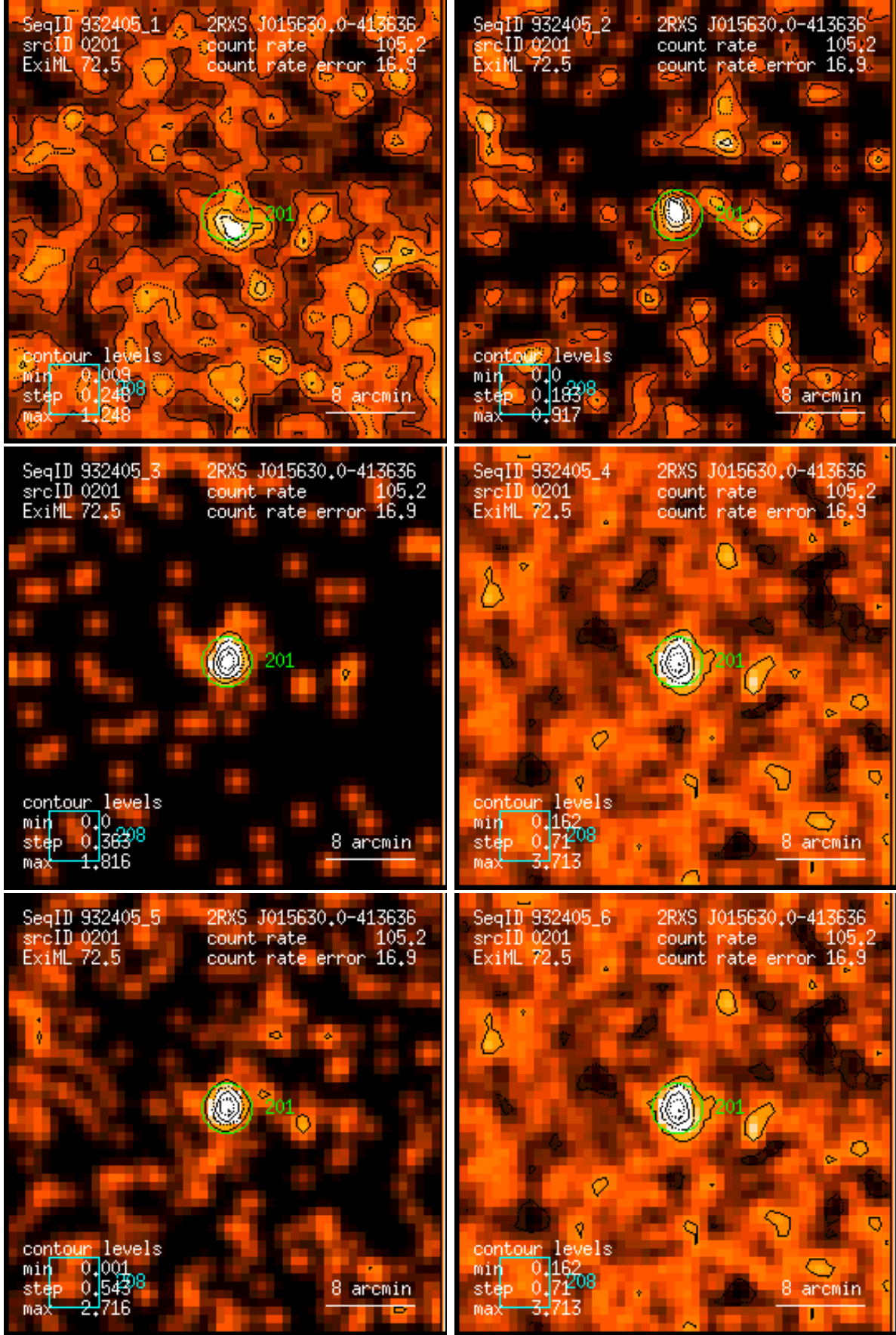
Figure 201: RASS 932405: detection 0201: band rate images, Gaussian filter: (1) PSPC channels 11 – 41, (2) 52 – 90, (3) 91 – 201, (4) 11 – 235, (5) 52 – 201, (6) 11 – 201. Broad band rates in counts/ks. Band rate contour levels in counts/ks/arcmin 2 .
