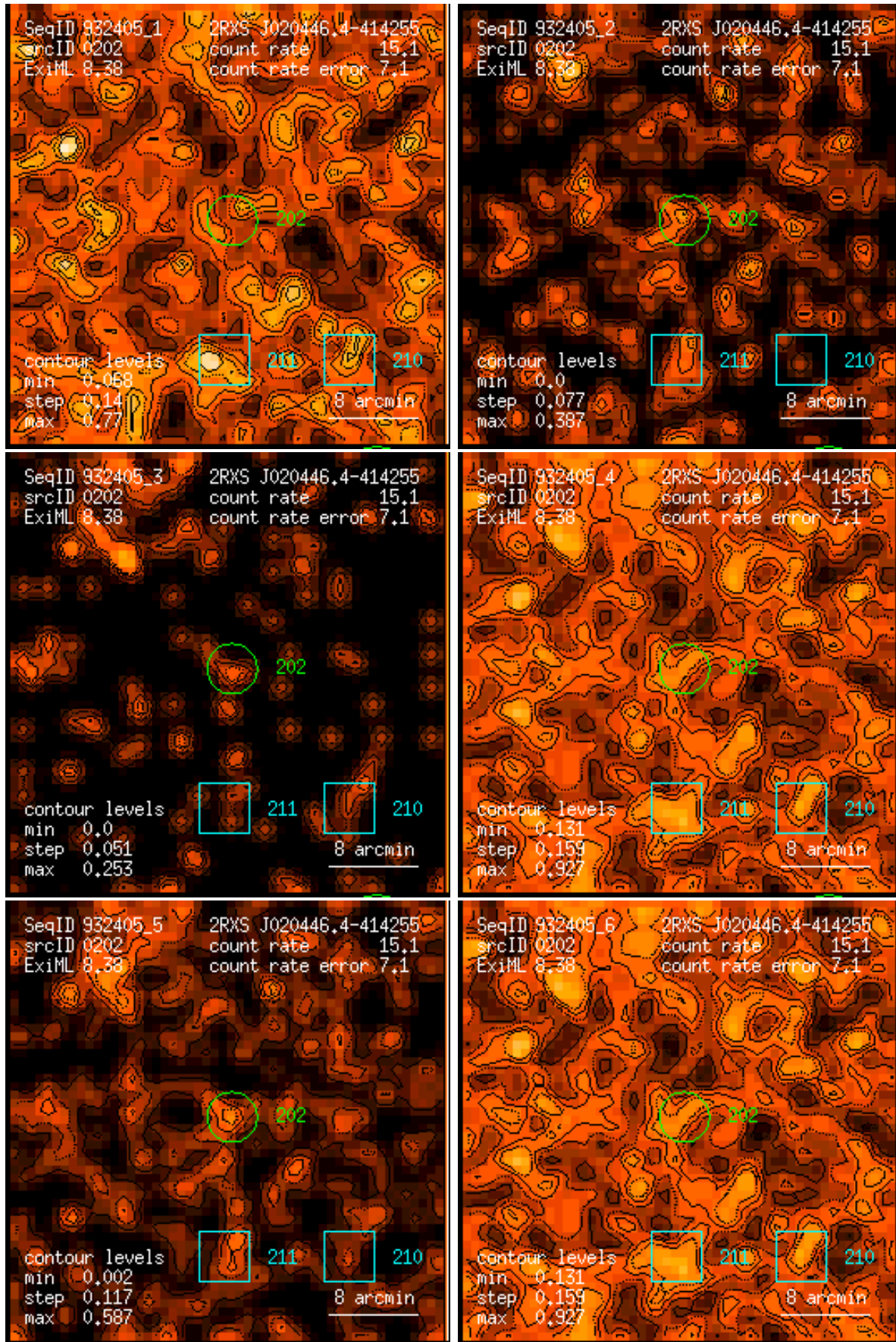
Figure 202: RASS 932405: detection 0202: band rate images, Gaussian filter: (1) PSPC channels 11 – 41, (2) 52 – 90, (3) 91 – 201, (4) 11 – 235, (5) 52 – 201, (6) 11 – 201. Broad band rates in counts/ks. Band rate contour levels in counts/ks/arcmin 2 .
