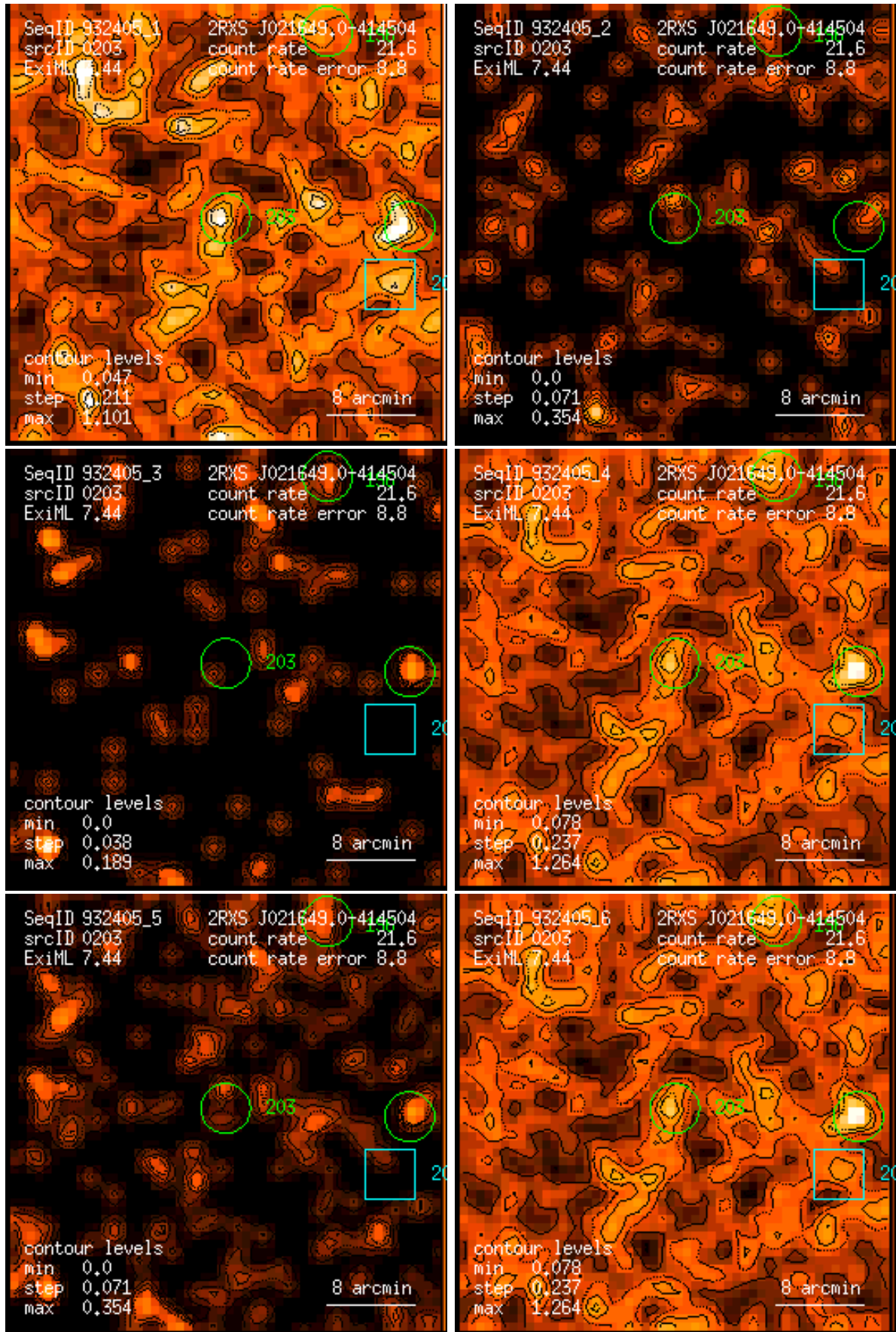
Figure 203: RASS 932405: detection 0203: band rate images, Gaussian filter: (1) PSPC channels 11 – 41, (2) 52 – 90, (3) 91 – 201, (4) 11 – 235, (5) 52 – 201, (6) 11 – 201. Broad band rates in counts/ks. Band rate contour levels in counts/ks/arcmin 2 .
