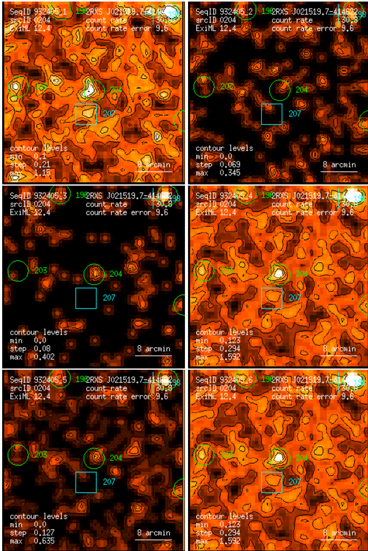
Figure 204: RASS 932405: detection 0204: band rate images, Gaussian filter: (1) PSPC channels 11 – 41, (2) 52 – 90, (3) 91 – 201, (4) 11 – 235, (5) 52 – 201, (6) 11 – 201. Broad band rates in counts/ks. Band rate contour levels in counts/ks/arcmin 2 .
