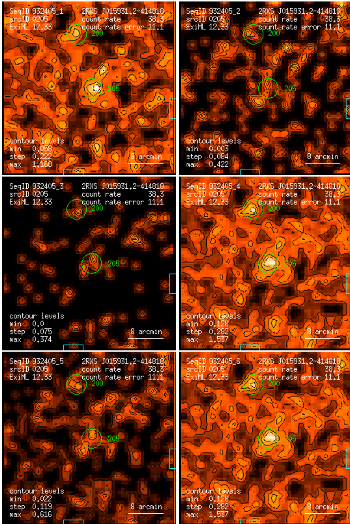
Figure 205: RASS 932405: detection 0205: band rate images, Gaussian filter: (1) PSPC channels 11 – 41, (2) 52 – 90, (3) 91 – 201, (4) 11 – 235, (5) 52 – 201, (6) 11 – 201. Broad band rates in counts/ks. Band rate contour levels in counts/ks/arcmin 2 .
