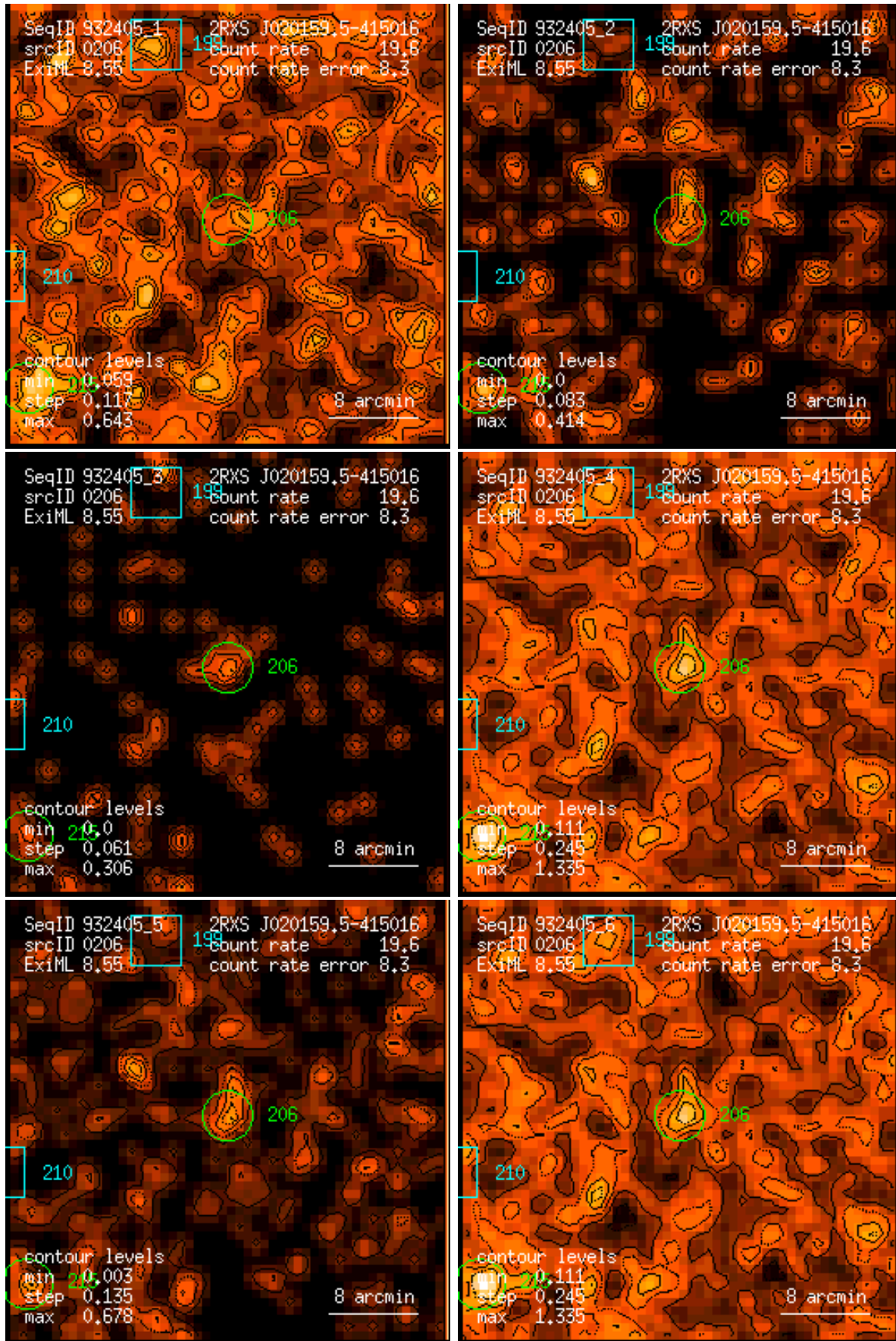
Figure 206: RASS 932405: detection 0206: band rate images, Gaussian filter: (1) PSPC channels 11 – 41, (2) 52 – 90, (3) 91 – 201, (4) 11 – 235, (5) 52 – 201, (6) 11 – 201. Broad band rates in counts/ks. Band rate contour levels in counts/ks/arcmin 2 .
