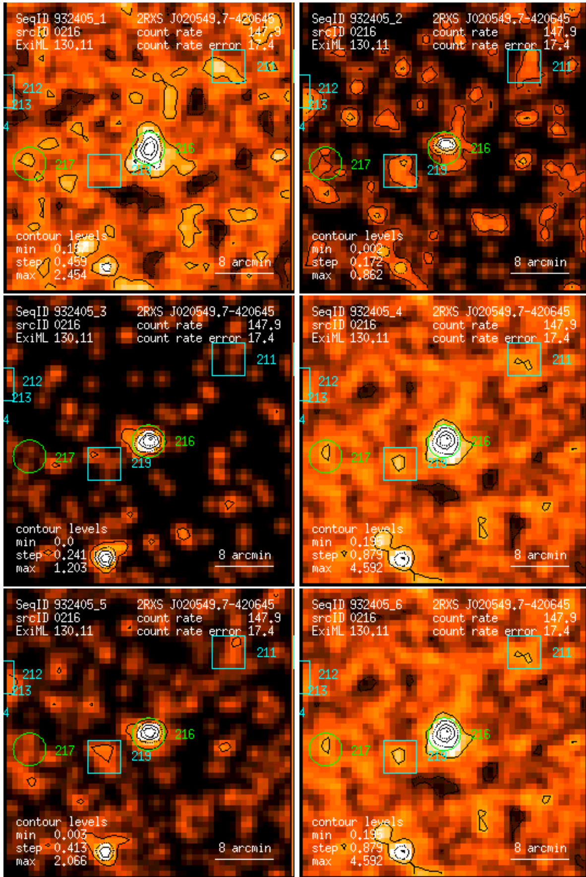
Figure 216: RASS 932405: detection 0216: band rate images, Gaussian filter: (1) PSPC channels 11 – 41, (2) 52 – 90, (3) 91 – 201, (4) 11 – 235, (5) 52 – 201, (6) 11 – 201. Broad band rates in counts/ks. Band rate contour levels in counts/ks/arcmin 2 .
