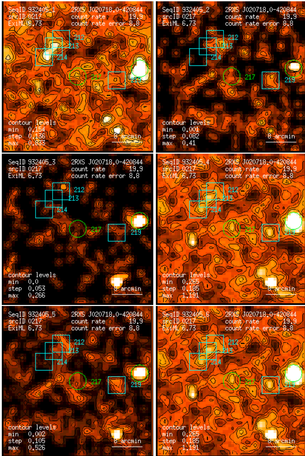
Figure 217: RASS 932405: detection 0217: band rate images, Gaussian filter: (1) PSPC channels 11 – 41, (2) 52 – 90, (3) 91 – 201, (4) 11 – 235, (5) 52 – 201, (6) 11 – 201. Broad band rates in counts/ks. Band rate contour levels in counts/ks/arcmin 2 .
