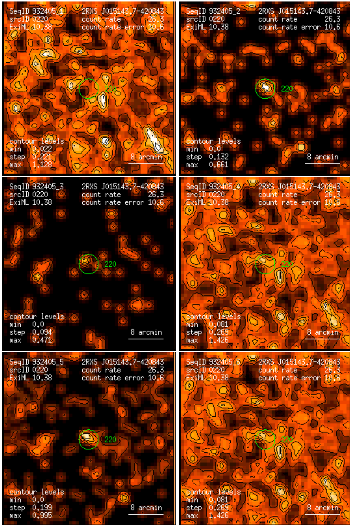
Figure 220: RASS 932405: detection 0220: band rate images, Gaussian filter: (1) PSPC channels 11 – 41, (2) 52 – 90, (3) 91 – 201, (4) 11 – 235, (5) 52 – 201, (6) 11 – 201. Broad band rates in counts/ks. Band rate contour levels in counts/ks/arcmin 2 .
