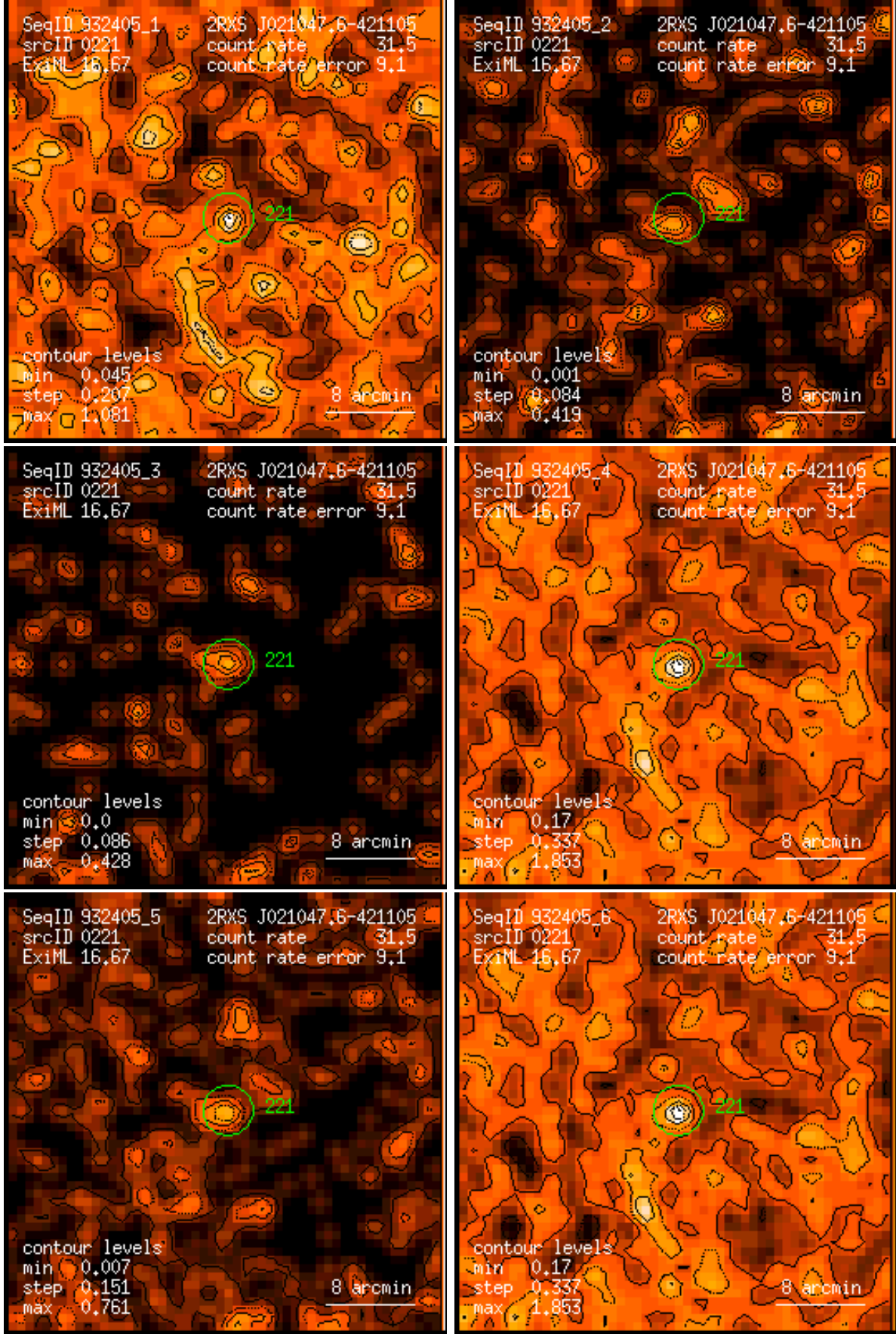
Figure 221: RASS 932405: detection 0221: band rate images, Gaussian filter: (1) PSPC channels 11 – 41, (2) 52 – 90, (3) 91 – 201, (4) 11 – 235, (5) 52 – 201, (6) 11 – 201. Broad band rates in counts/ks. Band rate contour levels in counts/ks/arcmin 2 .
