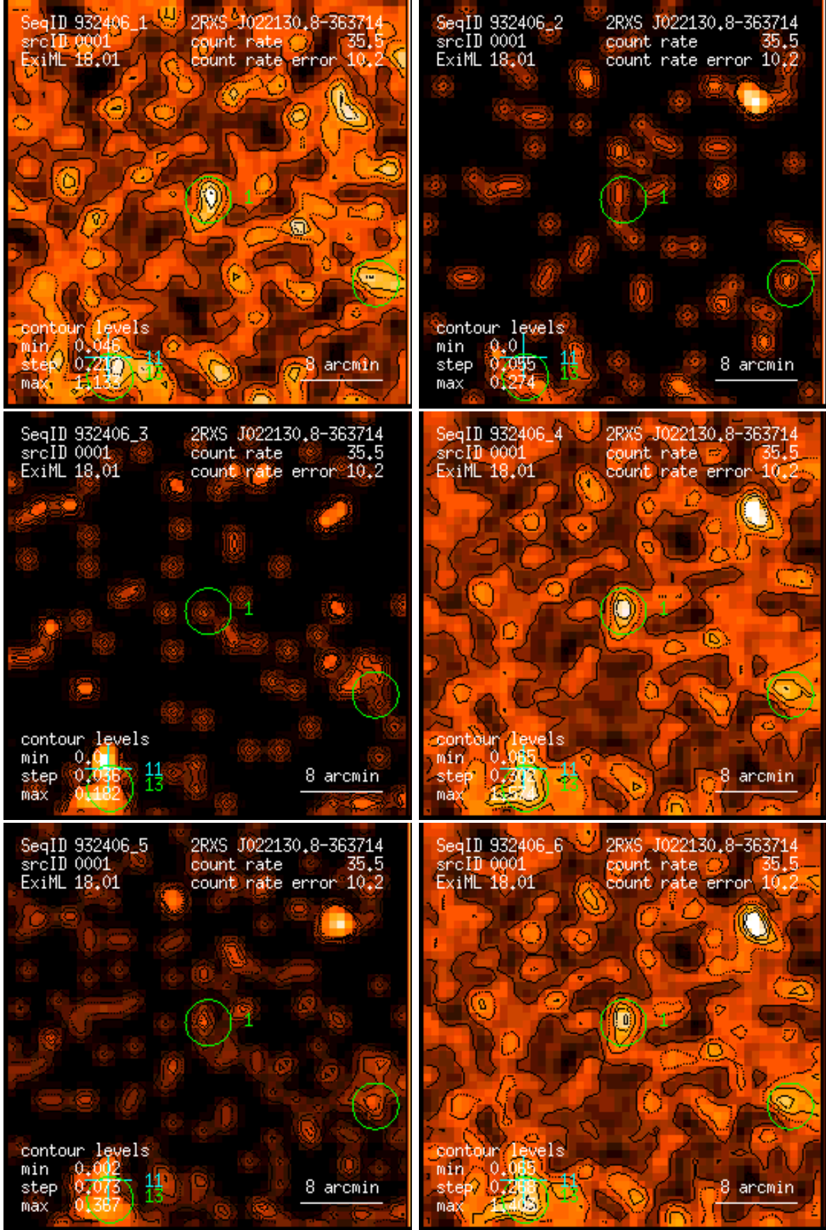
Figure 1: RASS 932406: detection 0001: band rate images, Gaussian filter: (1) PSPC channels 11 – 41, (2) 52 – 90, (3) 91 – 201, (4) 11 – 235, (5) 52 – 201, (6) 11 – 201. Broad band rates in counts/ks. Band rate contour levels in counts/ks/arcmin 2 .
