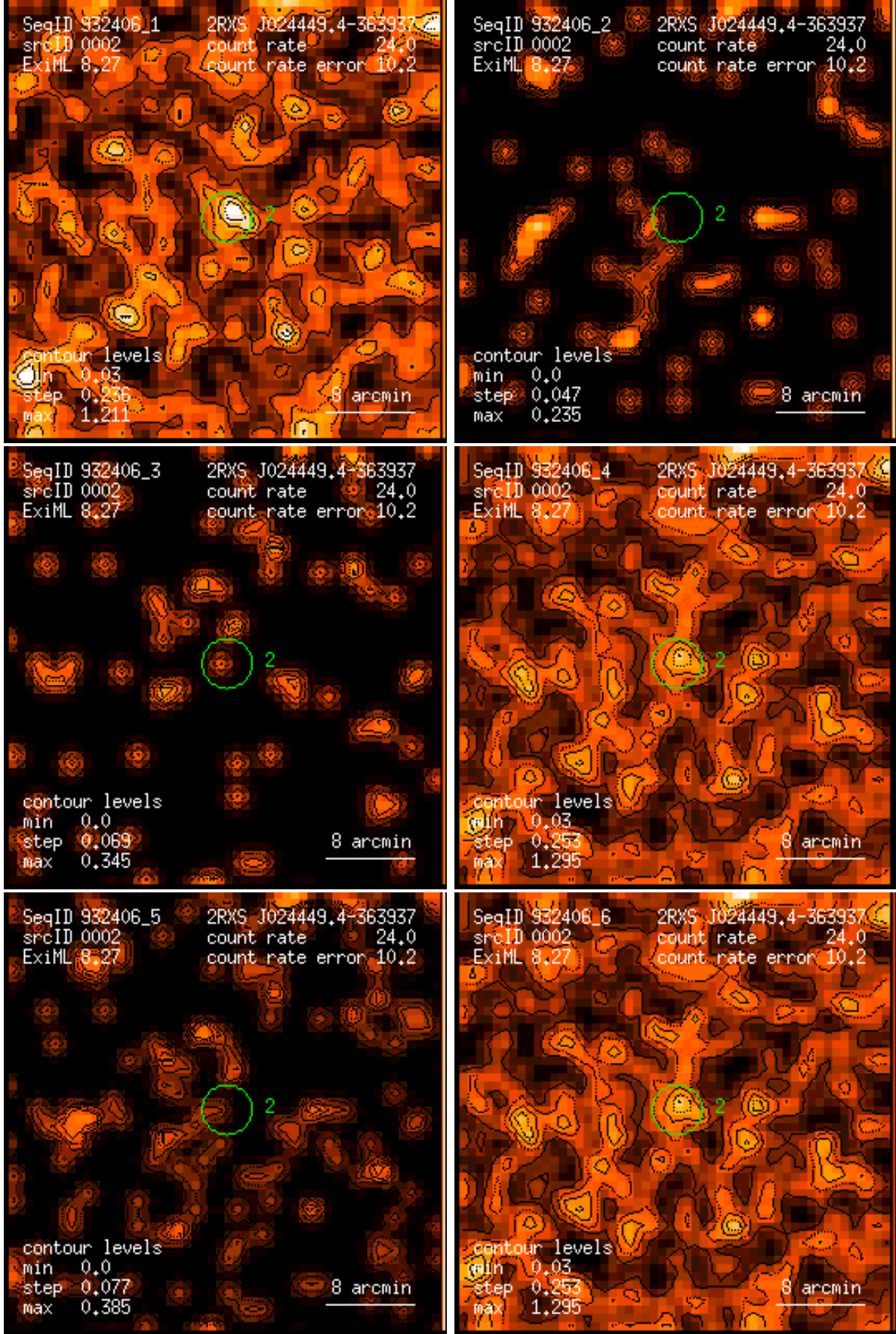
Figure 2: RASS 932406: detection 0002: band rate images, Gaussian filter: (1) PSPC channels 11 – 41, (2) 52 – 90, (3) 91 – 201, (4) 11 – 235, (5) 52 – 201, (6) 11 – 201. Broad band rates in counts/ks. Band rate contour levels in counts/ks/arcmin 2 .
