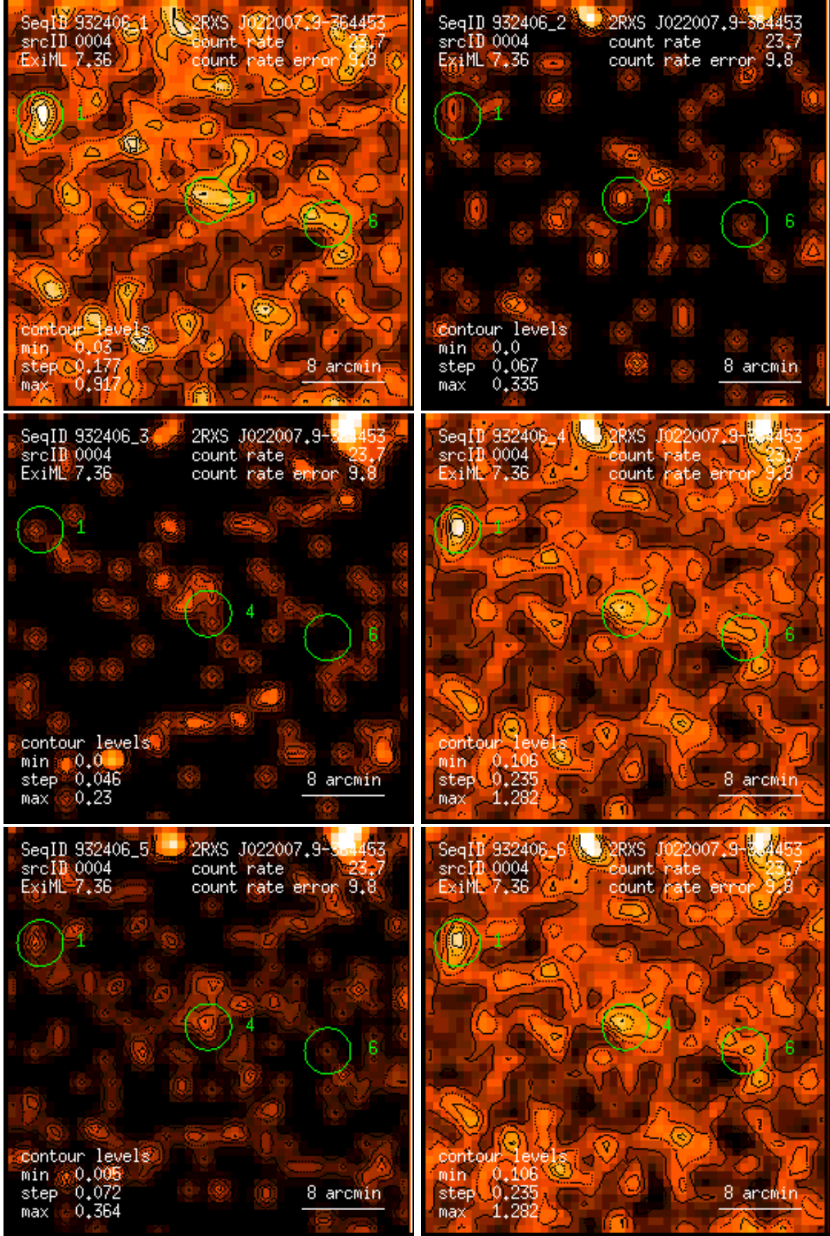
Figure 4: RASS 932406: detection 0004: band rate images, Gaussian filter: (1) PSPC channels 11 – 41, (2) 52 – 90, (3) 91 – 201, (4) 11 – 235, (5) 52 – 201, (6) 11 – 201. Broad band rates in counts/ks. Band rate contour levels in counts/ks/arcmin 2 .
