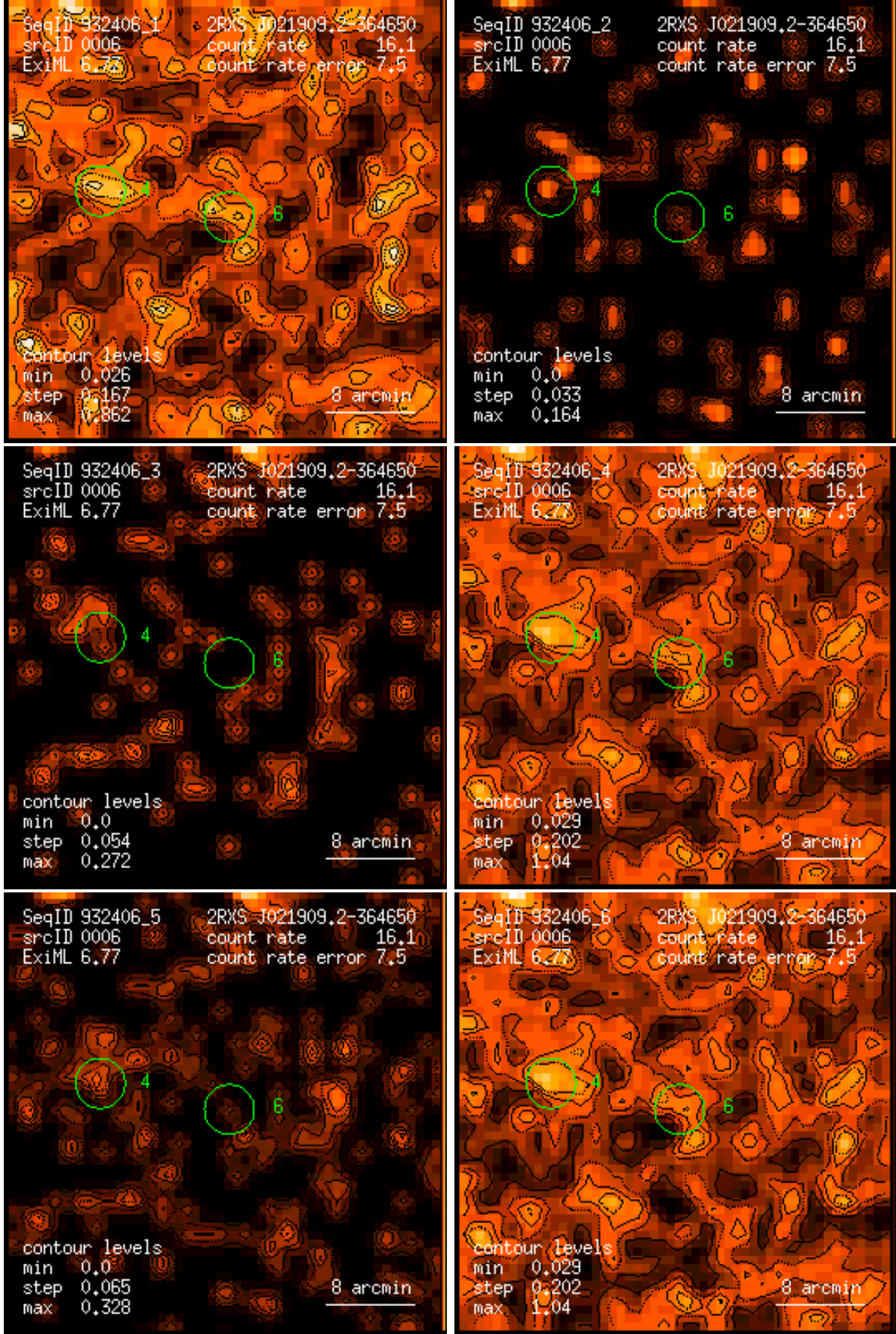
Figure 6: RASS 932406: detection 0006: band rate images, Gaussian filter: (1) PSPC channels 11 – 41, (2) 52 – 90, (3) 91 – 201, (4) 11 – 235, (5) 52 – 201, (6) 11 – 201. Broad band rates in counts/ks. Band rate contour levels in counts/ks/arcmin 2 .
