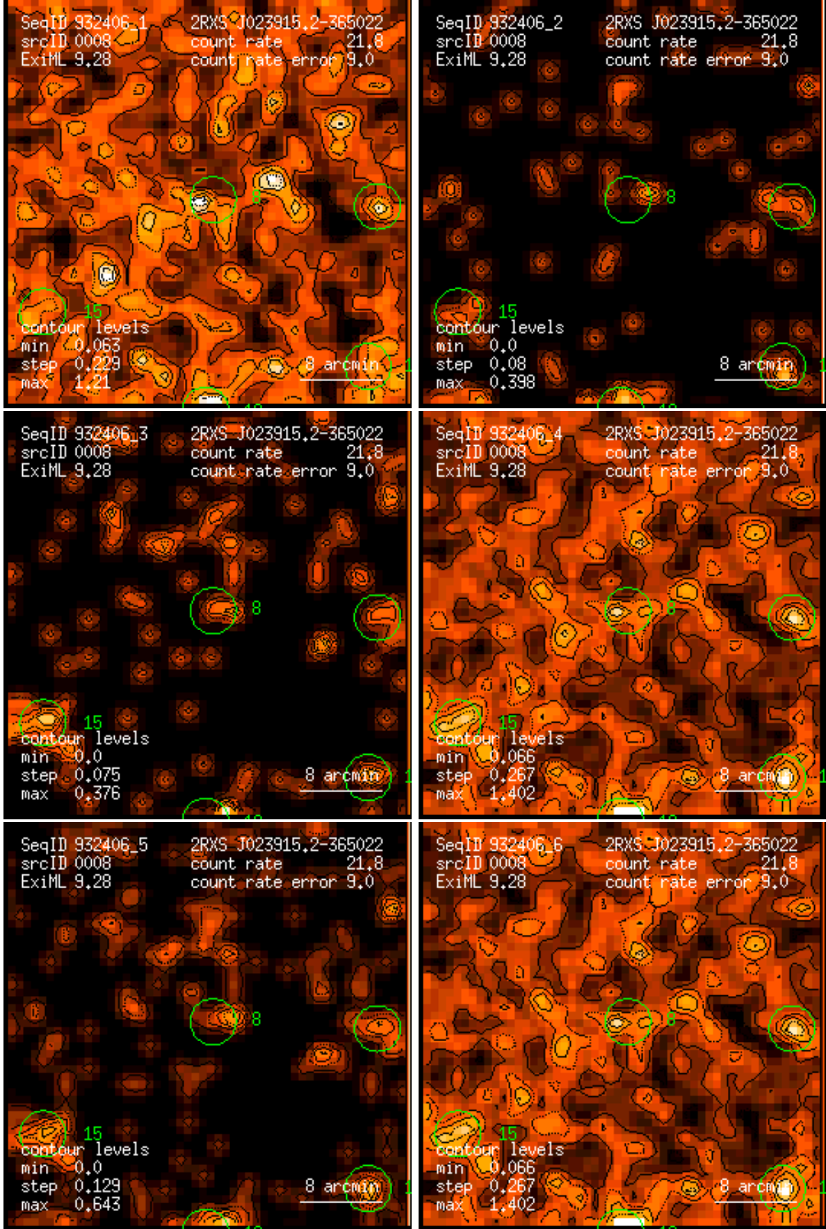
Figure 8: RASS 932406: detection 0008: band rate images, Gaussian filter: (1) PSPC channels 11 – 41, (2) 52 – 90, (3) 91 – 201, (4) 11 – 235, (5) 52 – 201, (6) 11 – 201. Broad band rates in counts/ks. Band rate contour levels in counts/ks/arcmin 2 .
