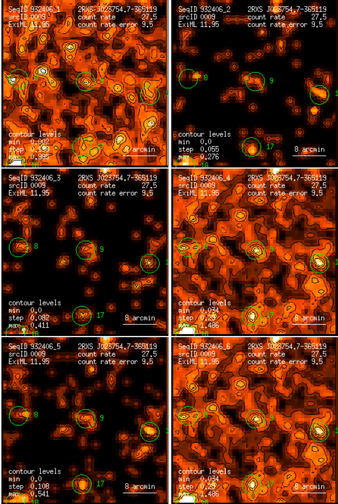
Figure 9: RASS 932406: detection 0009: band rate images, Gaussian filter: (1) PSPC channels 11 – 41, (2) 52 – 90, (3) 91 – 201, (4) 11 – 235, (5) 52 – 201, (6) 11 – 201. Broad band rates in counts/ks. Band rate contour levels in counts/ks/arcmin 2 .
