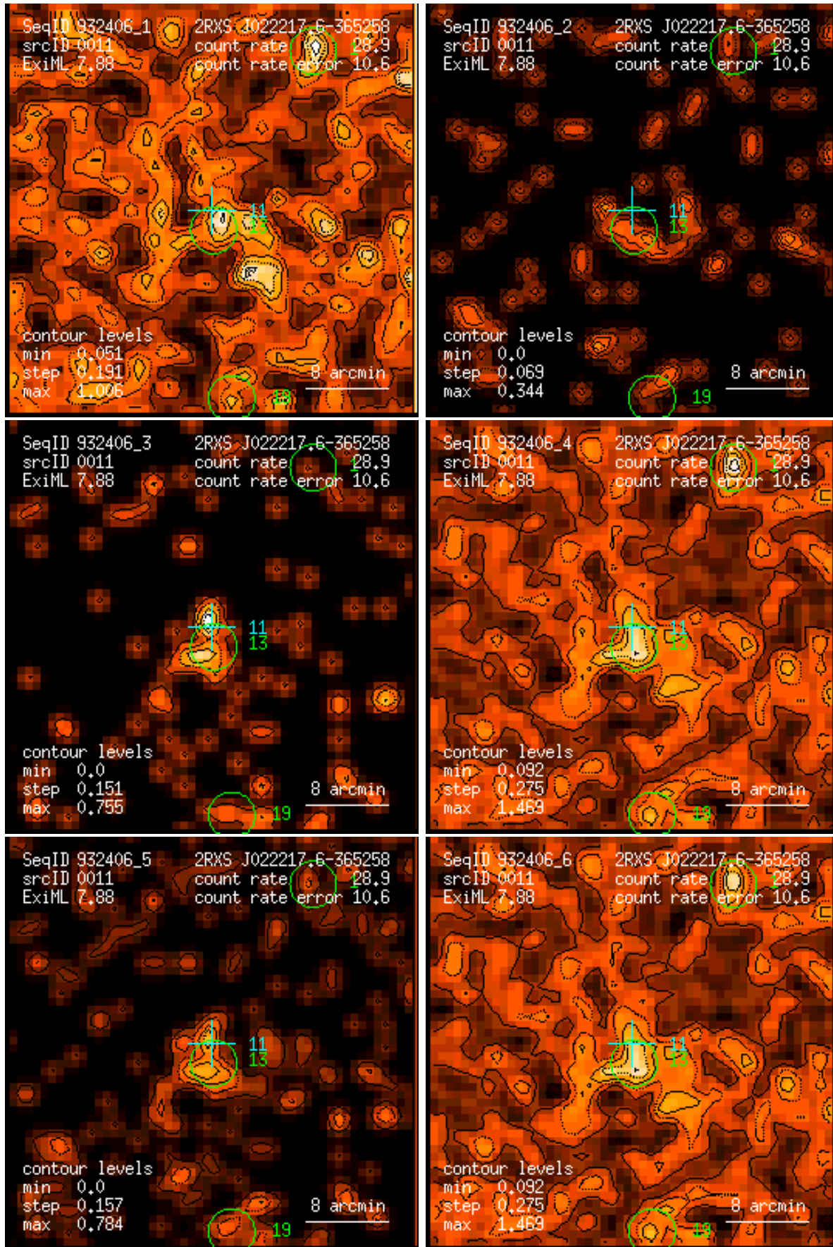
Figure 11: RASS 932406: detection 0011: band rate images, Gaussian filter: (1) PSPC channels 11 – 41, (2) 52 – 90, (3) 91 – 201, (4) 11 – 235, (5) 52 – 201, (6) 11 – 201. Broad band rates in counts/ks. Band rate contour levels in counts/ks/arcmin 2 .
