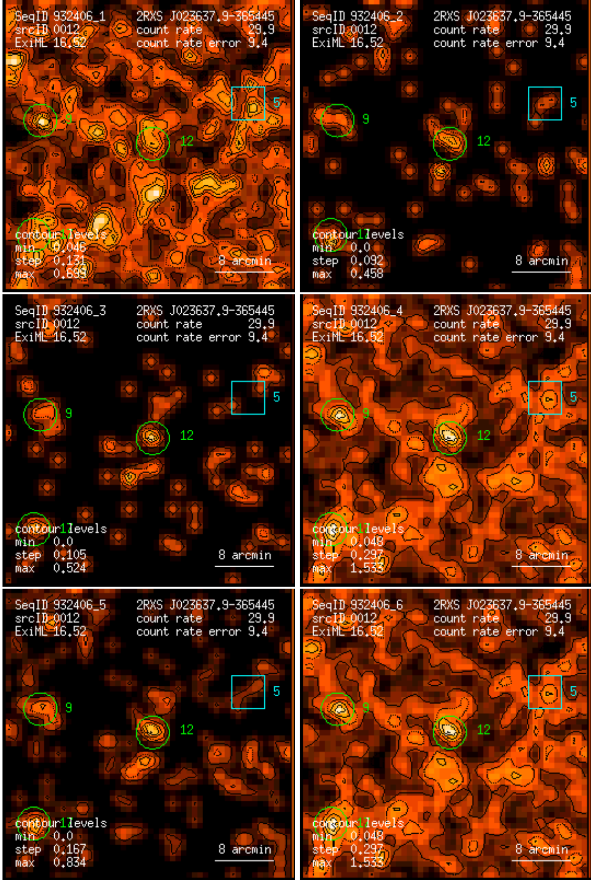
Figure 12: RASS 932406: detection 0012: band rate images, Gaussian filter: (1) PSPC channels 11 – 41, (2) 52 – 90, (3) 91 – 201, (4) 11 – 235, (5) 52 – 201, (6) 11 – 201. Broad band rates in counts/ks. Band rate contour levels in counts/ks/arcmin 2 .
