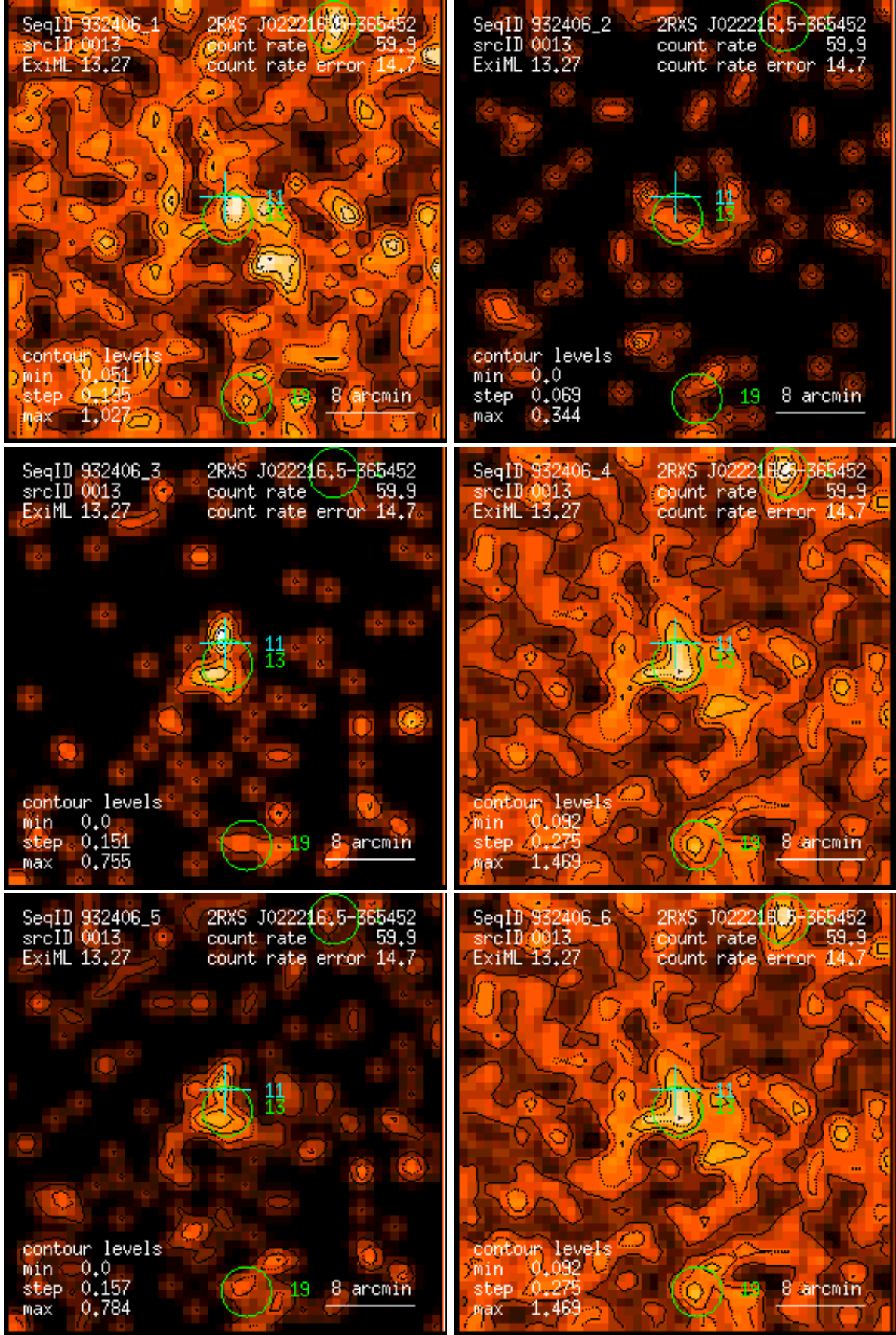
Figure 13: RASS 932406: detection 0013: band rate images, Gaussian filter: (1) PSPC channels 11 – 41, (2) 52 – 90, (3) 91 – 201, (4) 11 – 235, (5) 52 – 201, (6) 11 – 201. Broad band rates in counts/ks. Band rate contour levels in counts/ks/arcmin 2 .
