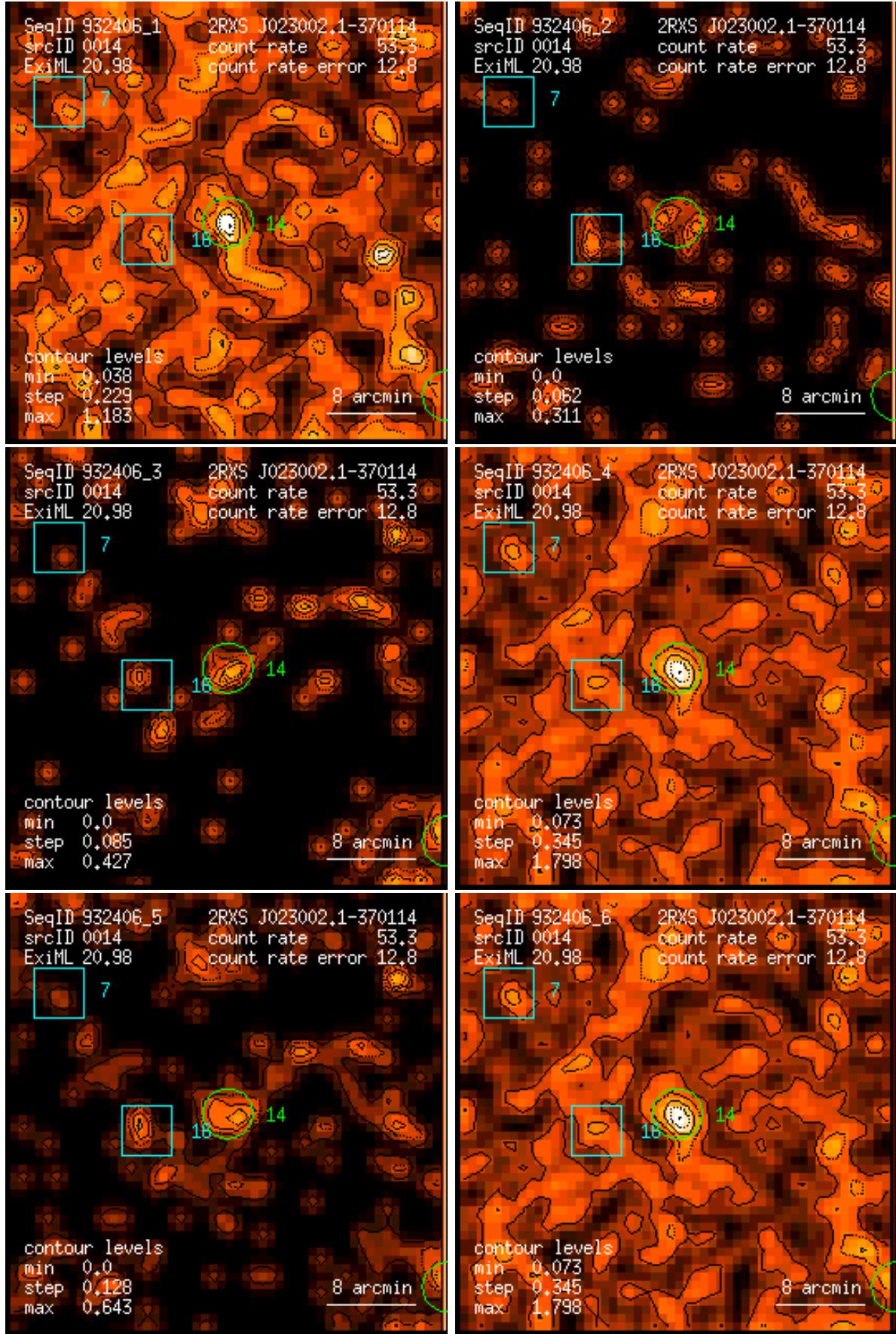
Figure 14: RASS 932406: detection 0014: band rate images, Gaussian filter: (1) PSPC channels 11 – 41, (2) 52 – 90, (3) 91 – 201, (4) 11 – 235, (5) 52 – 201, (6) 11 – 201. Broad band rates in counts/ks. Band rate contour levels in counts/ks/arcmin 2 .
