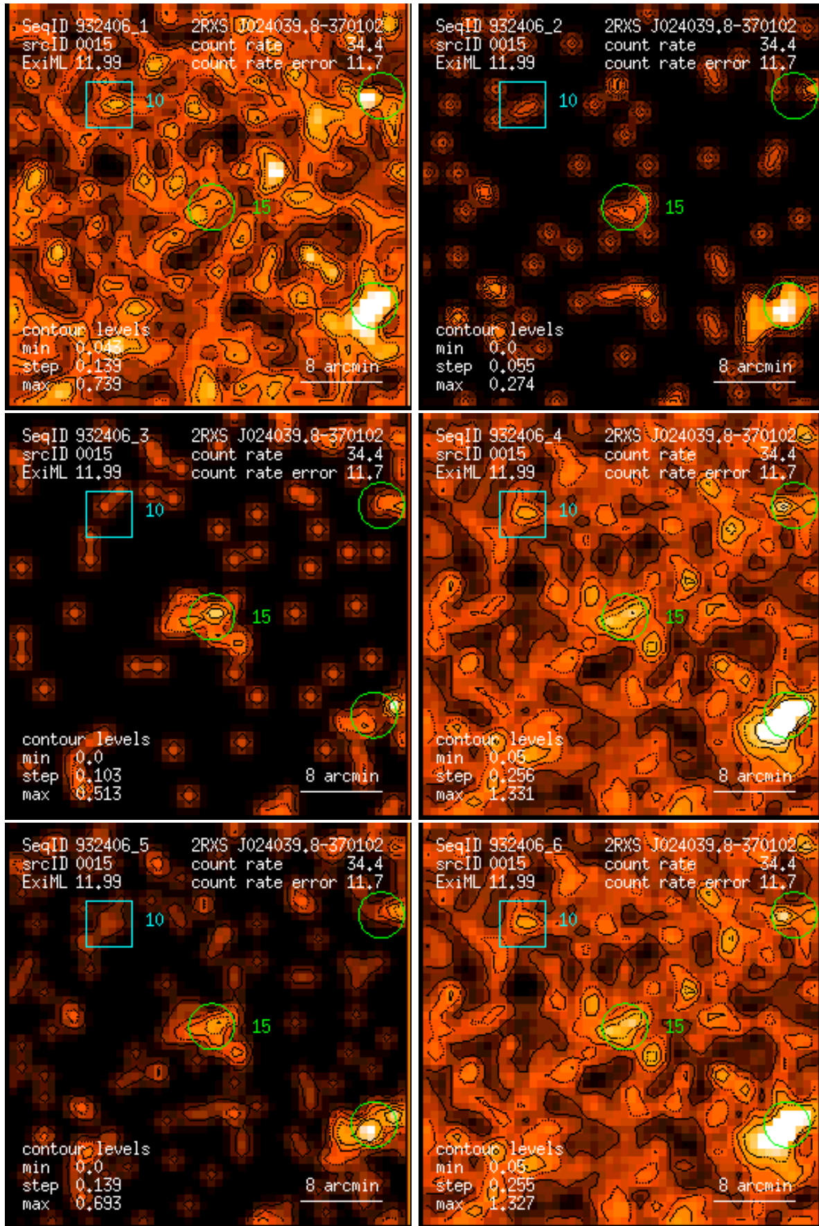
Figure 15: RASS 932406: detection 0015: band rate images, Gaussian filter: (1) PSPC channels 11 – 41, (2) 52 – 90, (3) 91 – 201, (4) 11 – 235, (5) 52 – 201, (6) 11 – 201. Broad band rates in counts/ks. Band rate contour levels in counts/ks/arcmin 2 .
