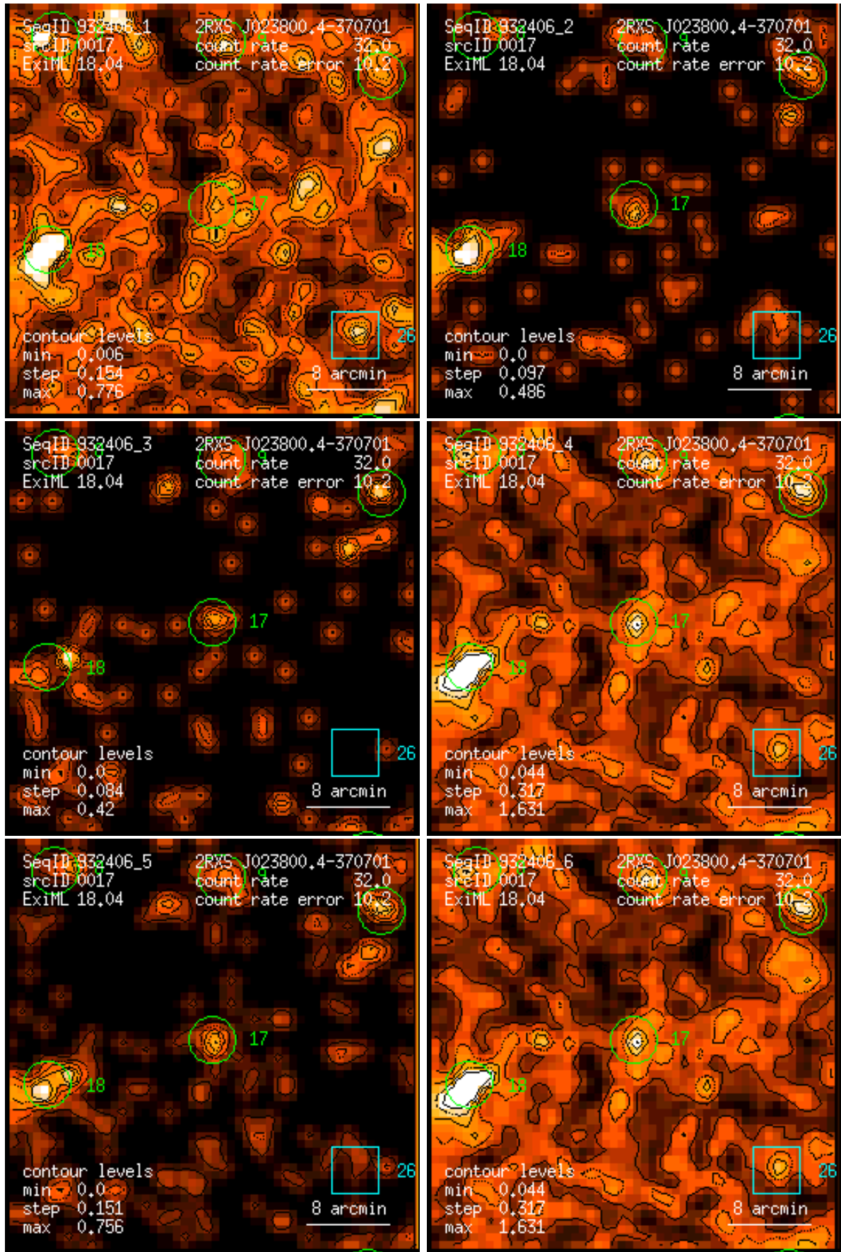
Figure 17: RASS 932406: detection 0017: band rate images, Gaussian filter: (1) PSPC channels 11 – 41, (2) 52 – 90, (3) 91 – 201, (4) 11 – 235, (5) 52 – 201, (6) 11 – 201. Broad band rates in counts/ks. Band rate contour levels in counts/ks/arcmin 2 .
