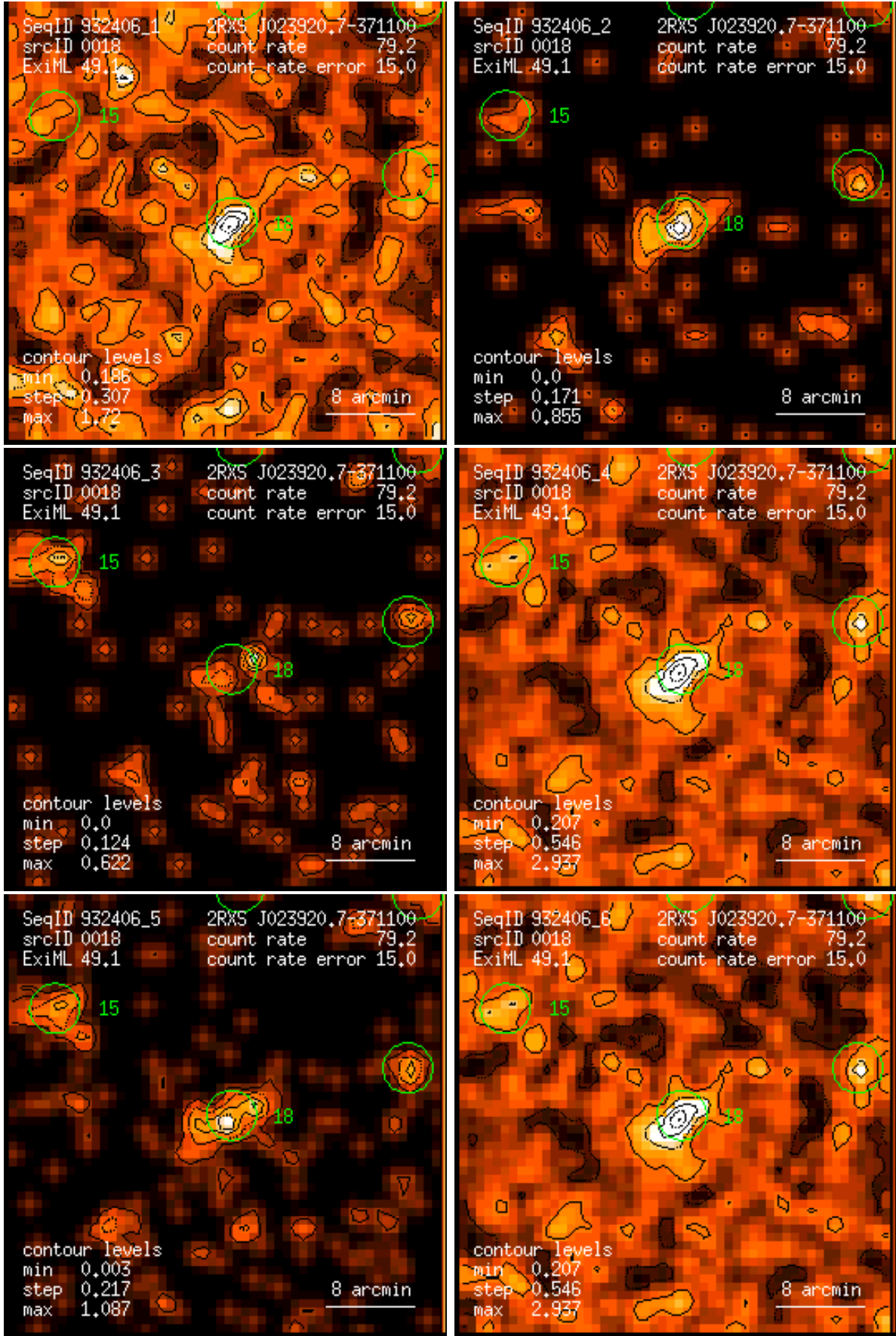
Figure 18: RASS 932406: detection 0018: band rate images, Gaussian filter: (1) PSPC channels 11 – 41, (2) 52 – 90, (3) 91 – 201, (4) 11 – 235, (5) 52 – 201, (6) 11 – 201. Broad band rates in counts/ks. Band rate contour levels in counts/ks/arcmin 2 .
