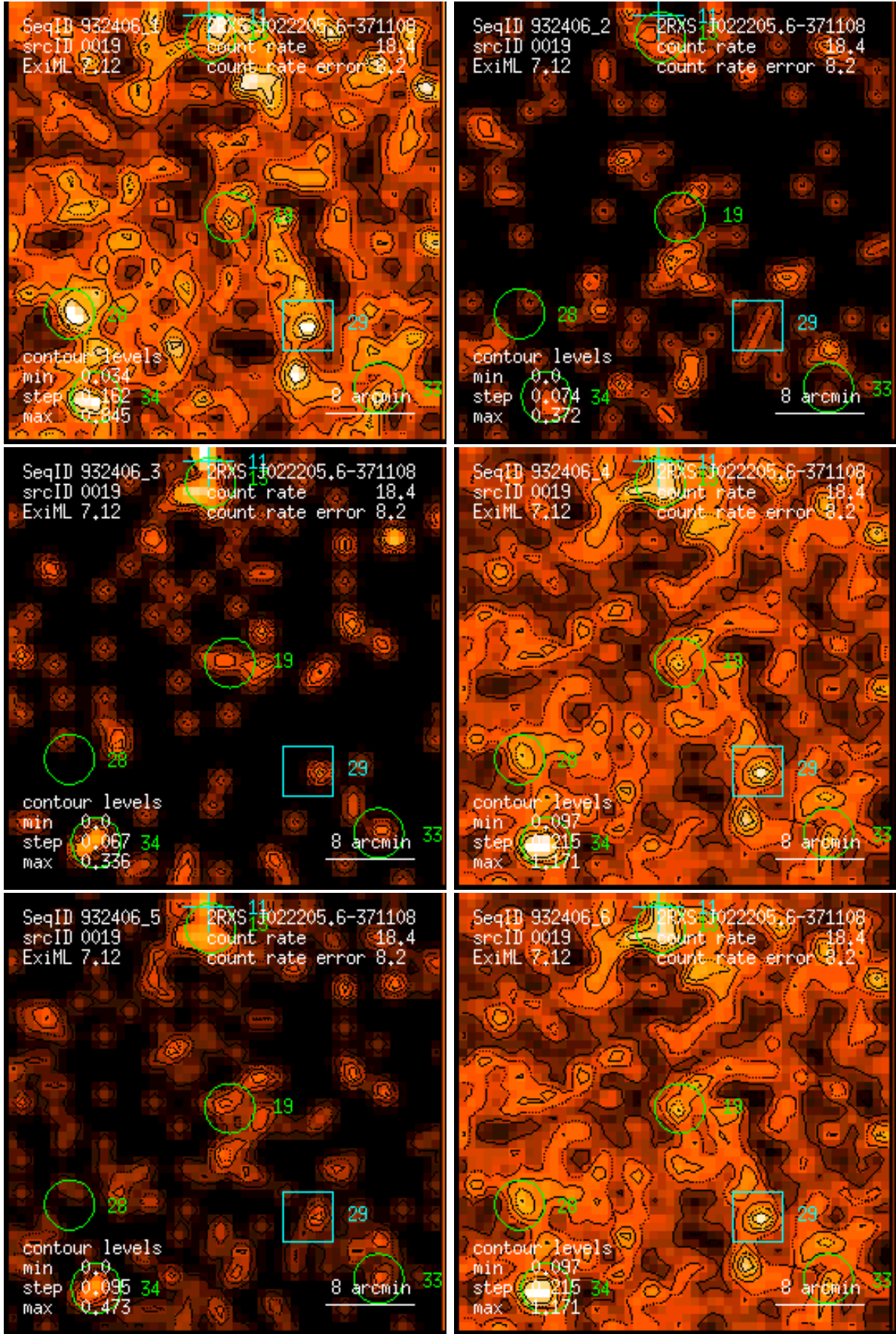
Figure 19: RASS 932406: detection 0019: band rate images, Gaussian filter: (1) PSPC channels 11 – 41, (2) 52 – 90, (3) 91 – 201, (4) 11 – 235, (5) 52 – 201, (6) 11 – 201. Broad band rates in counts/ks. Band rate contour levels in counts/ks/arcmin 2 .
