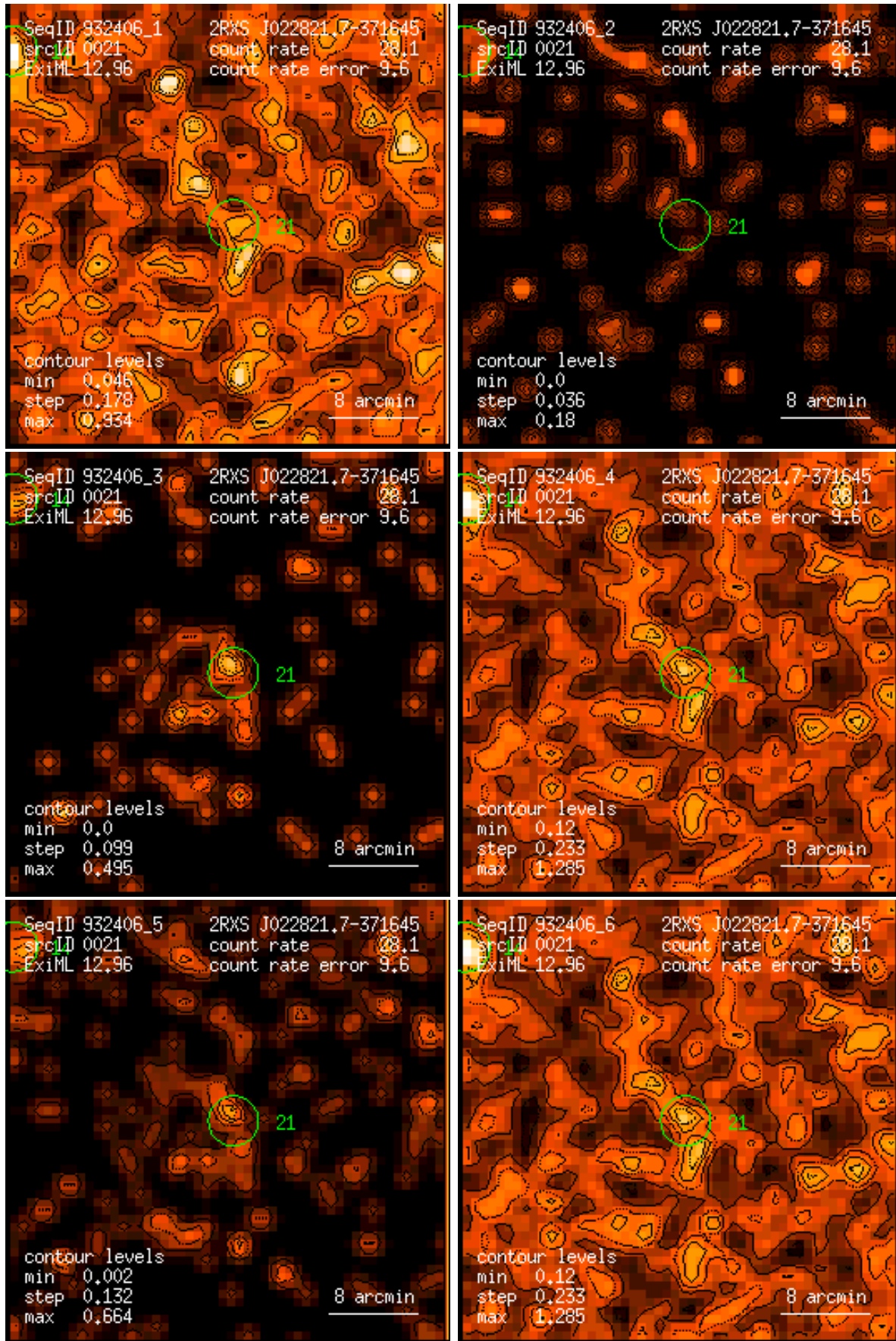
Figure 21: RASS 932406: detection 0021: band rate images, Gaussian filter: (1) PSPC channels 11 – 41, (2) 52 – 90, (3) 91 – 201, (4) 11 – 235, (5) 52 – 201, (6) 11 – 201. Broad band rates in counts/ks. Band rate contour levels in counts/ks/arcmin 2 .
