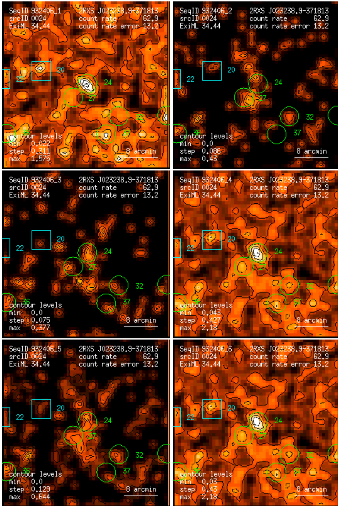
Figure 24: RASS 932406: detection 0024: band rate images, Gaussian filter: (1) PSPC channels 11 – 41, (2) 52 – 90, (3) 91 – 201, (4) 11 – 235, (5) 52 – 201, (6) 11 – 201. Broad band rates in counts/ks. Band rate contour levels in counts/ks/arcmin 2 .
