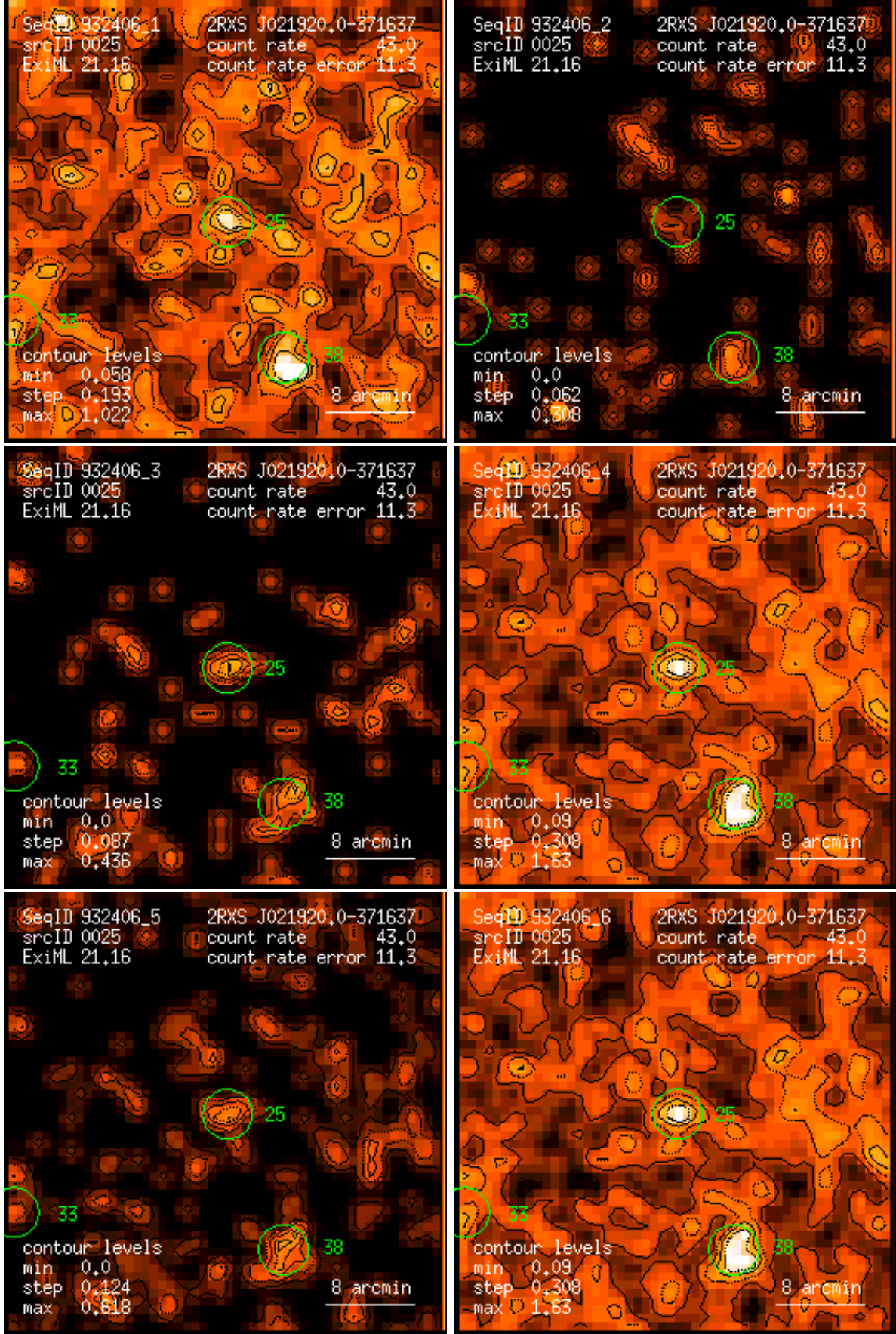
Figure 25: RASS 932406: detection 0025: band rate images, Gaussian filter: (1) PSPC channels 11 – 41, (2) 52 – 90, (3) 91 – 201, (4) 11 – 235, (5) 52 – 201, (6) 11 – 201. Broad band rates in counts/ks. Band rate contour levels in counts/ks/arcmin 2 .
