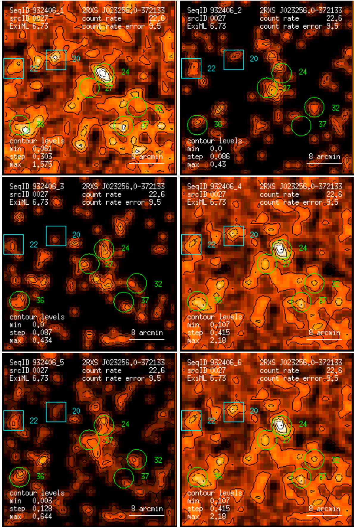
Figure 27: RASS 932406: detection 0027: band rate images, Gaussian filter: (1) PSPC channels 11 – 41, (2) 52 – 90, (3) 91 – 201, (4) 11 – 235, (5) 52 – 201, (6) 11 – 201. Broad band rates in counts/ks. Band rate contour levels in counts/ks/arcmin 2 .
