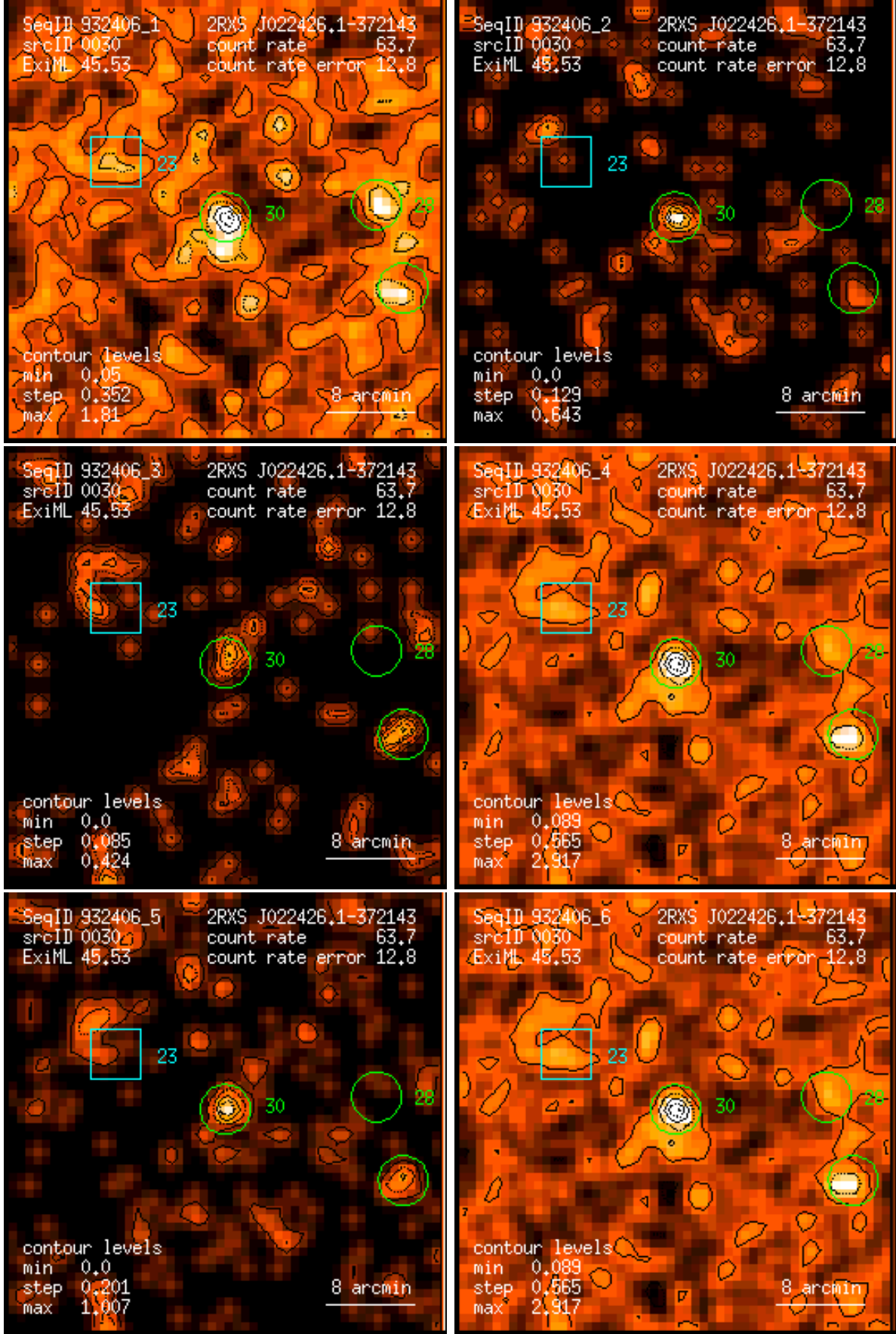
Figure 30: RASS 932406: detection 0030: band rate images, Gaussian filter: (1) PSPC channels 11 – 41, (2) 52 – 90, (3) 91 – 201, (4) 11 – 235, (5) 52 – 201, (6) 11 – 201. Broad band rates in counts/ks. Band rate contour levels in counts/ks/arcmin 2 .
