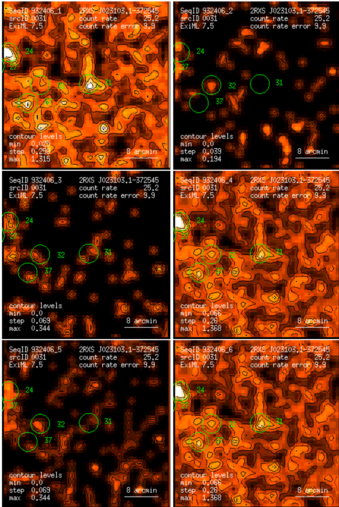
Figure 31: RASS 932406: detection 0031: band rate images, Gaussian filter: (1) PSPC channels 11 – 41, (2) 52 – 90, (3) 91 – 201, (4) 11 – 235, (5) 52 – 201, (6) 11 – 201. Broad band rates in counts/ks. Band rate contour levels in counts/ks/arcmin 2 .
