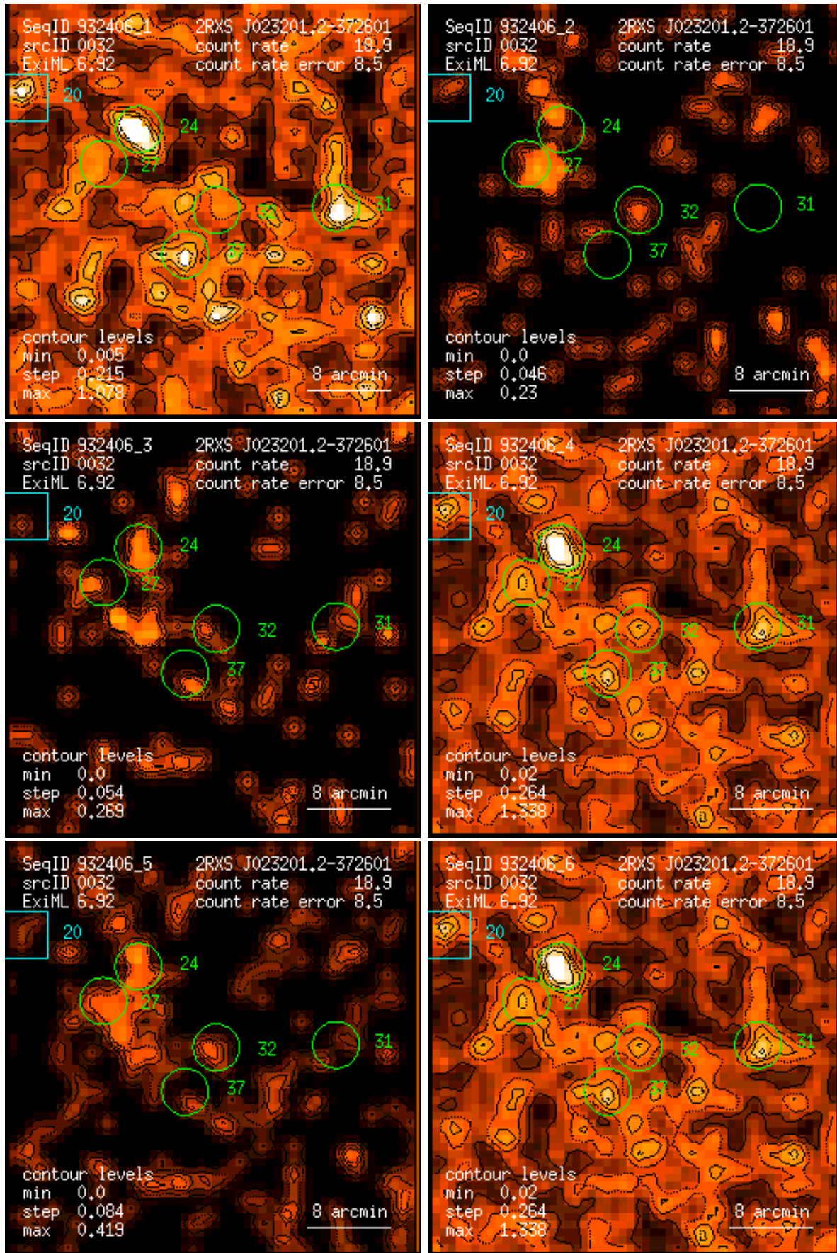
Figure 32: RASS 932406: detection 0032: band rate images, Gaussian filter: (1) PSPC channels 11 – 41, (2) 52 – 90, (3) 91 – 201, (4) 11 – 235, (5) 52 – 201, (6) 11 – 201. Broad band rates in counts/ks. Band rate contour levels in counts/ks/arcmin 2 .
