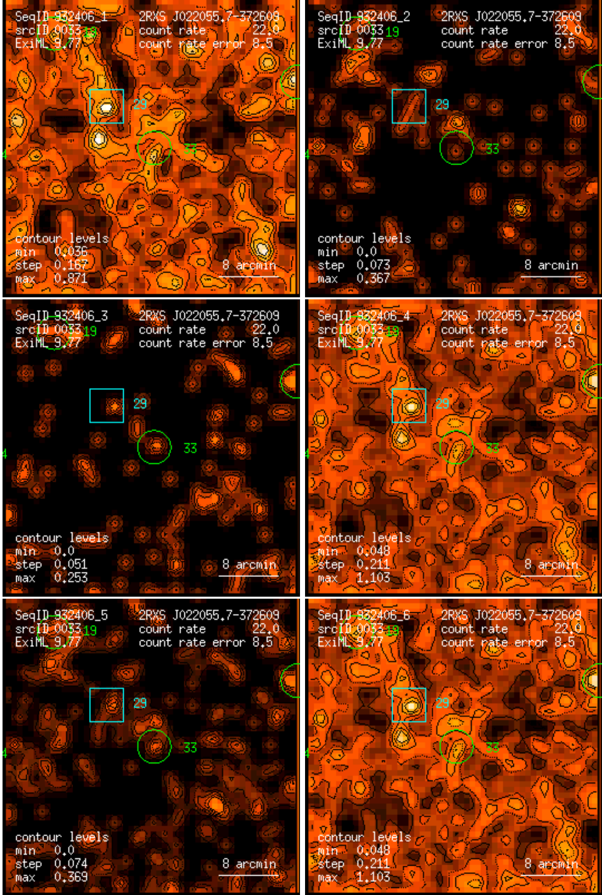
Figure 33: RASS 932406: detection 0033: band rate images, Gaussian filter: (1) PSPC channels 11 – 41, (2) 52 – 90, (3) 91 – 201, (4) 11 – 235, (5) 52 – 201, (6) 11 – 201. Broad band rates in counts/ks. Band rate contour levels in counts/ks/arcmin 2 .
