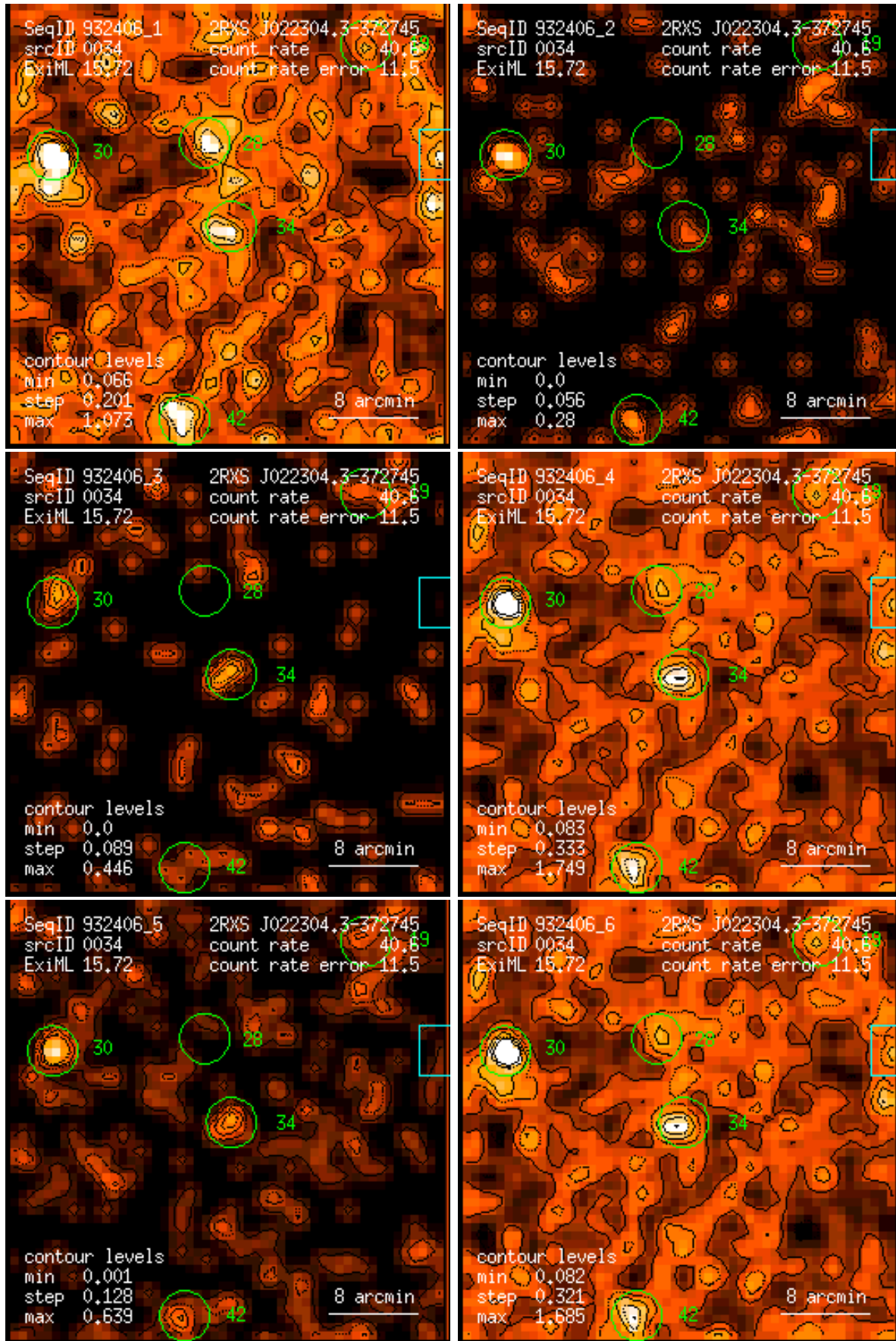
Figure 34: RASS 932406: detection 0034: band rate images, Gaussian filter: (1) PSPC channels 11 – 41, (2) 52 – 90, (3) 91 – 201, (4) 11 – 235, (5) 52 – 201, (6) 11 – 201. Broad band rates in counts/ks. Band rate contour levels in counts/ks/arcmin 2 .
