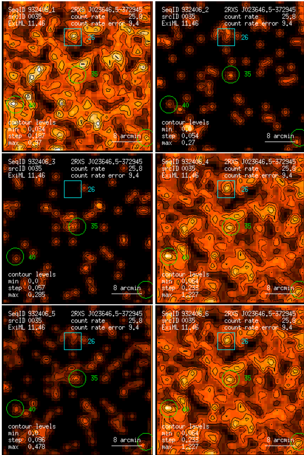
Figure 35: RASS 932406: detection 0035: band rate images, Gaussian filter: (1) PSPC channels 11 – 41, (2) 52 – 90, (3) 91 – 201, (4) 11 – 235, (5) 52 – 201, (6) 11 – 201. Broad band rates in counts/ks. Band rate contour levels in counts/ks/arcmin 2 .
