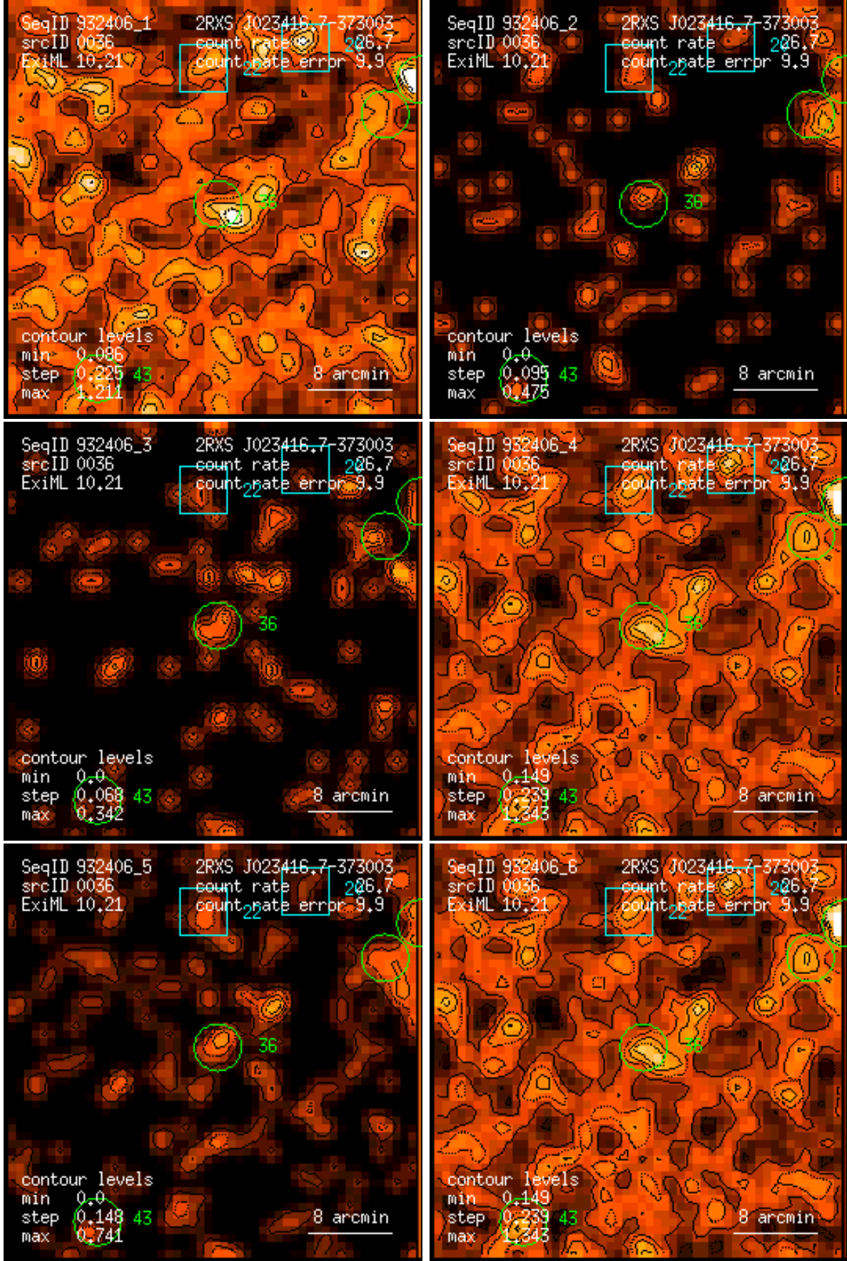
Figure 36: RASS 932406: detection 0036: band rate images, Gaussian filter: (1) PSPC channels 11 – 41, (2) 52 – 90, (3) 91 – 201, (4) 11 – 235, (5) 52 – 201, (6) 11 – 201. Broad band rates in counts/ks. Band rate contour levels in counts/ks/arcmin 2 .
