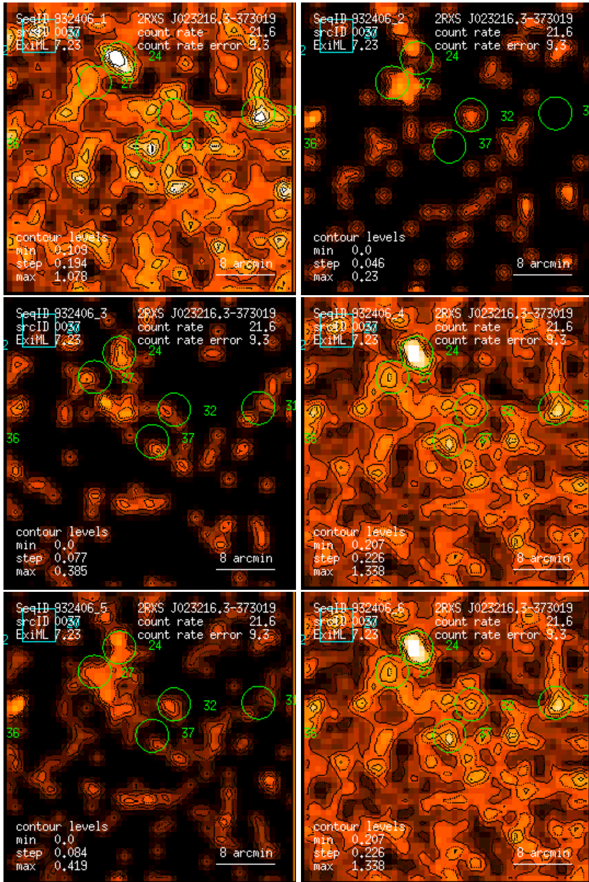
Figure 37: RASS 932406: detection 0037: band rate images, Gaussian filter: (1) PSPC channels 11 – 41, (2) 52 – 90, (3) 91 – 201, (4) 11 – 235, (5) 52 – 201, (6) 11 – 201. Broad band rates in counts/ks. Band rate contour levels in counts/ks/arcmin 2 .
