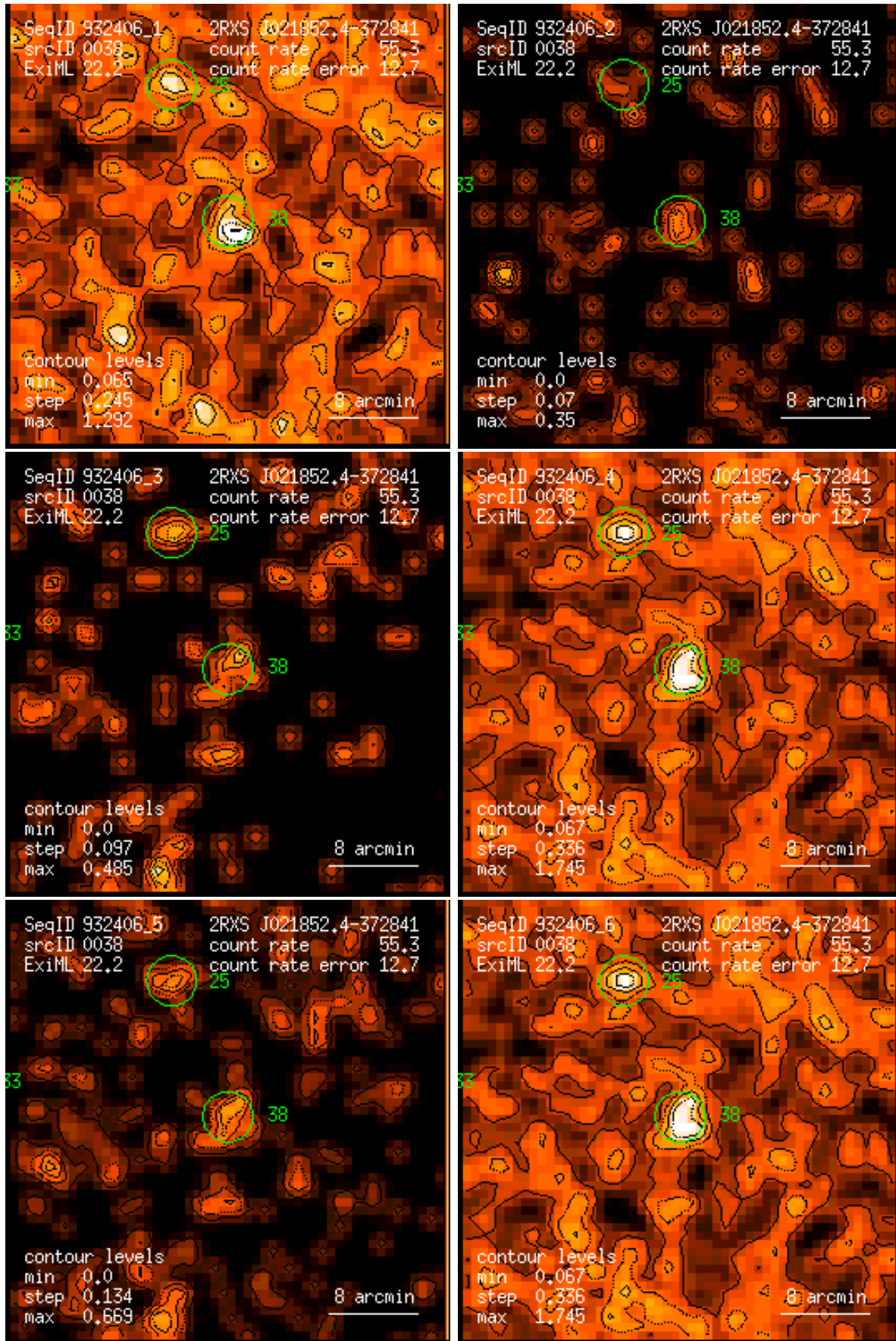
Figure 38: RASS 932406: detection 0038: band rate images, Gaussian filter: (1) PSPC channels 11 – 41, (2) 52 – 90, (3) 91 – 201, (4) 11 – 235, (5) 52 – 201, (6) 11 – 201. Broad band rates in counts/ks. Band rate contour levels in counts/ks/arcmin 2 .
