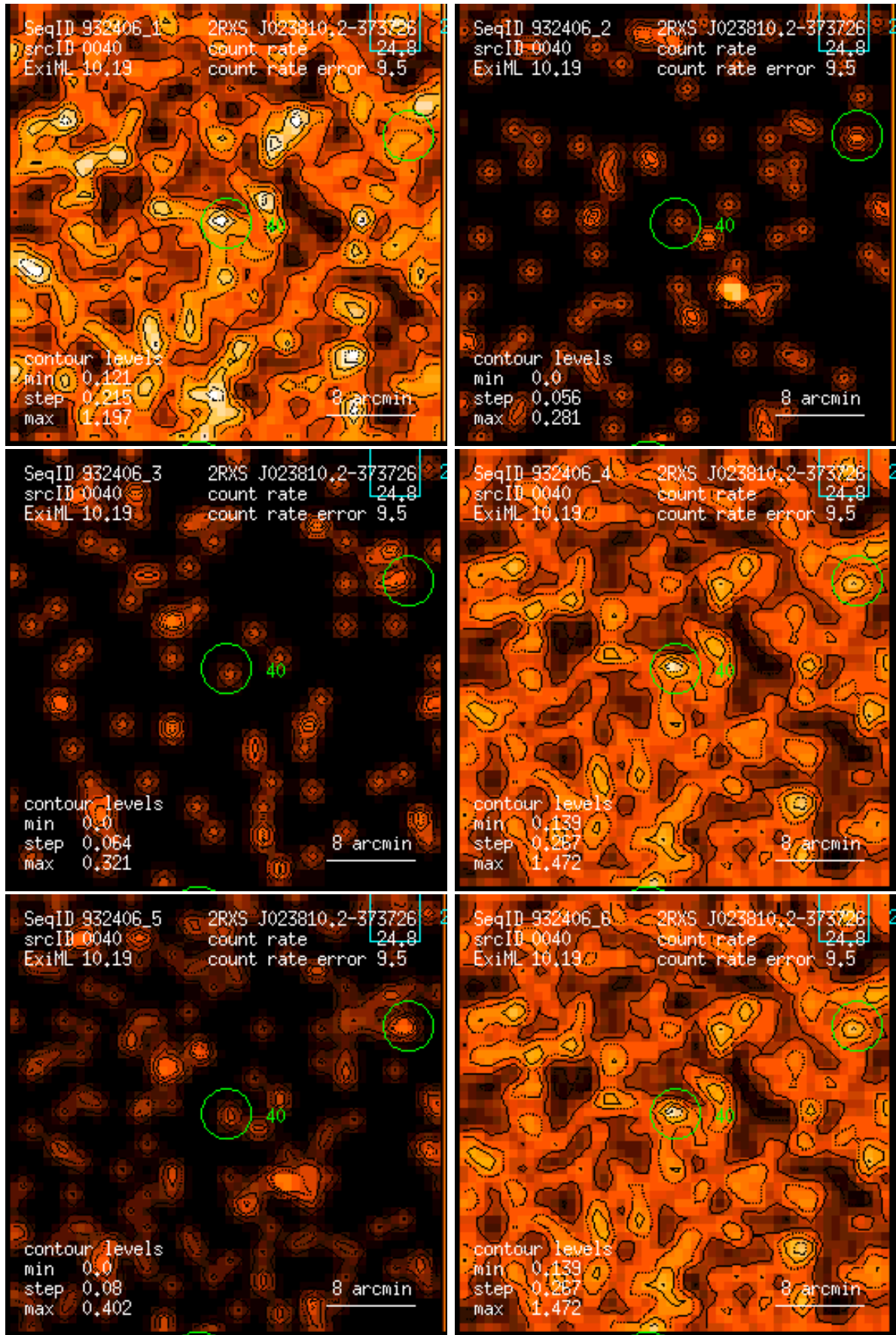
Figure 40: RASS 932406: detection 0040: band rate images, Gaussian filter: (1) PSPC channels 11 – 41, (2) 52 – 90, (3) 91 – 201, (4) 11 – 235, (5) 52 – 201, (6) 11 – 201. Broad band rates in counts/ks. Band rate contour levels in counts/ks/arcmin 2 .
