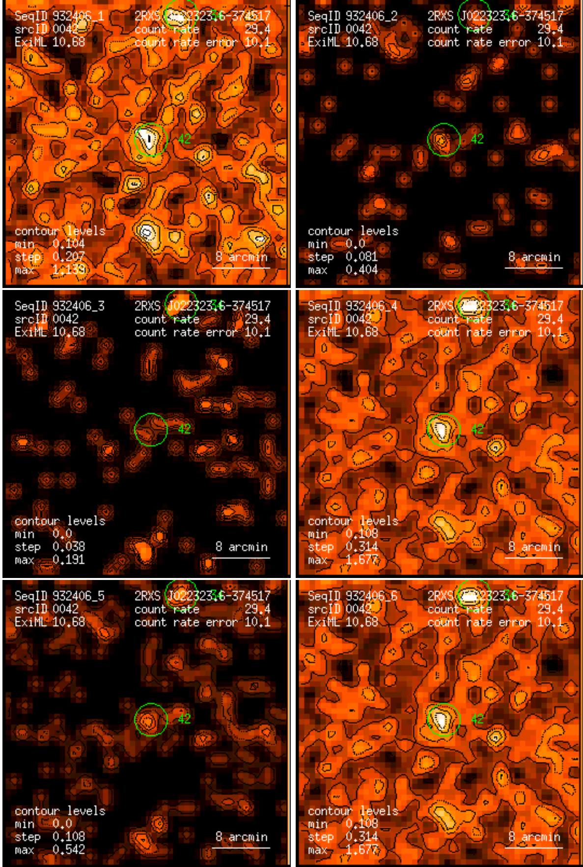
Figure 42: RASS 932406: detection 0042: band rate images, Gaussian filter: (1) PSPC channels 11 – 41, (2) 52 – 90, (3) 91 – 201, (4) 11 – 235, (5) 52 – 201, (6) 11 – 201. Broad band rates in counts/ks. Band rate contour levels in counts/ks/arcmin 2 .
