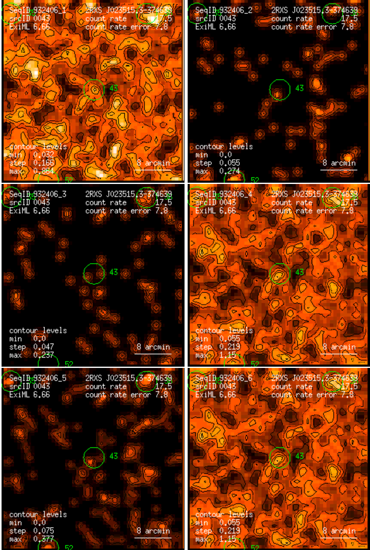
Figure 43: RASS 932406: detection 0043: band rate images, Gaussian filter: (1) PSPC channels 11 – 41, (2) 52 – 90, (3) 91 – 201, (4) 11 – 235, (5) 52 – 201, (6) 11 – 201. Broad band rates in counts/ks. Band rate contour levels in counts/ks/arcmin 2 .
