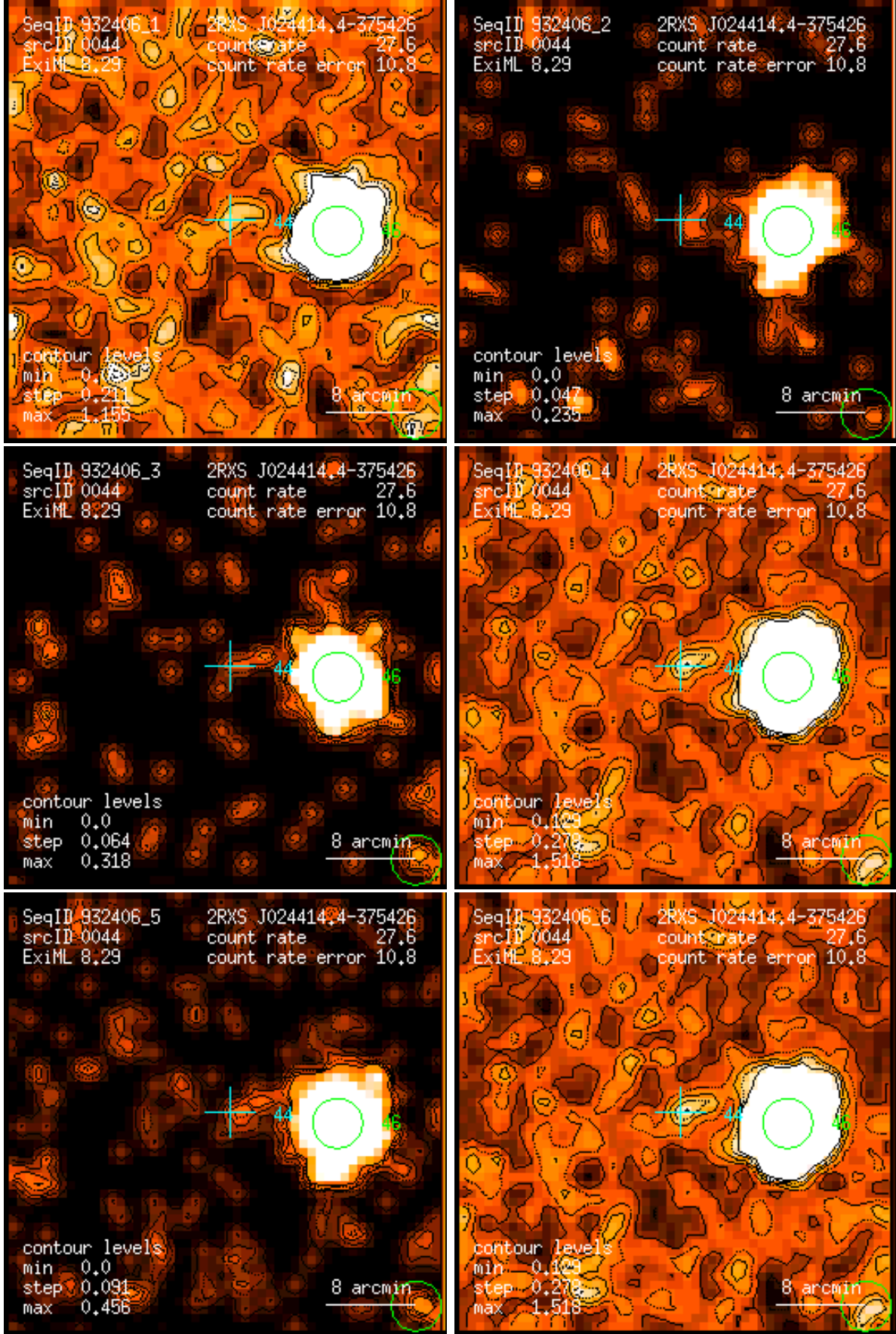
Figure 44: RASS 932406: detection 0044: band rate images, Gaussian filter: (1) PSPC channels 11 – 41, (2) 52 – 90, (3) 91 – 201, (4) 11 – 235, (5) 52 – 201, (6) 11 – 201. Broad band rates in counts/ks. Band rate contour levels in counts/ks/arcmin 2 .
